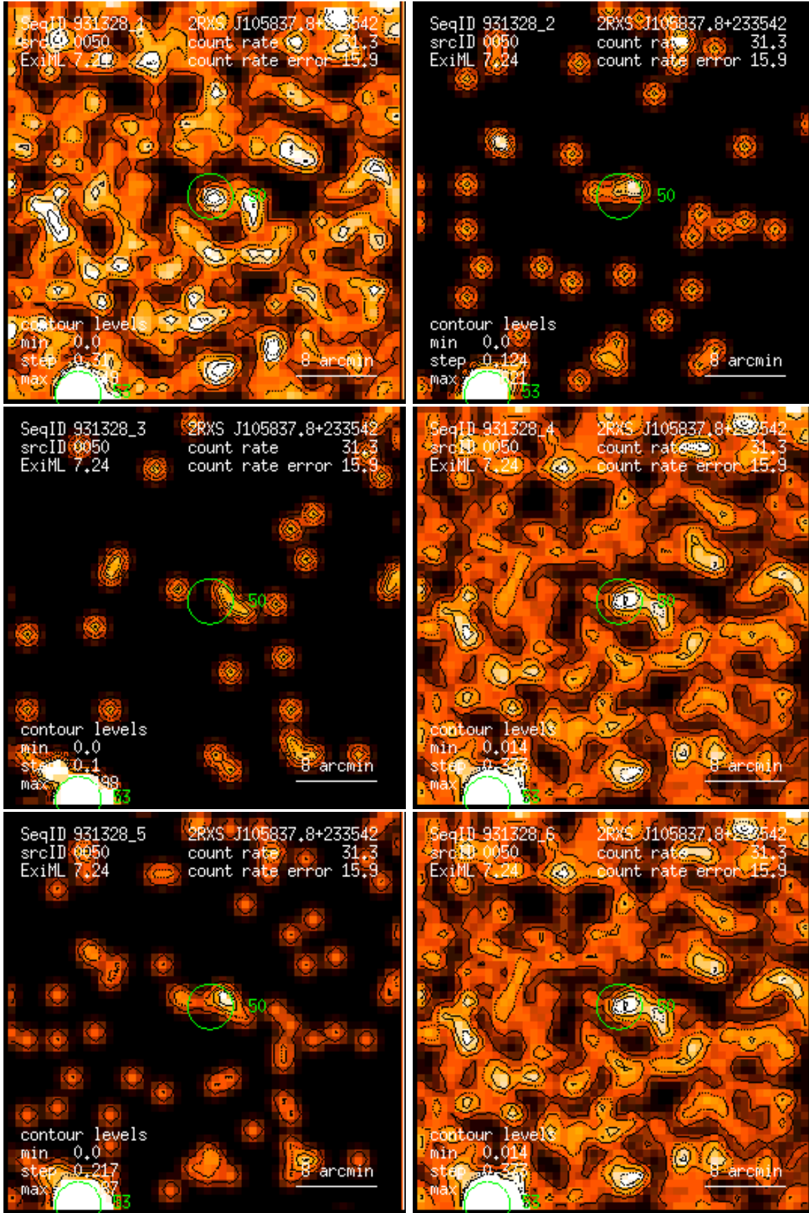
Figure 50: RASS 931328: detection 0050: band rate images, Gaussian filter: (1) PSPC channels 11 – 41, (2) 52 – 90, (3) 91 – 201, (4) 11 – 235, (5) 52 – 201, (6) 11 – 201. Broad band rates in counts/ks. Band rate contour levels in counts/ks/arcmin 2 .
