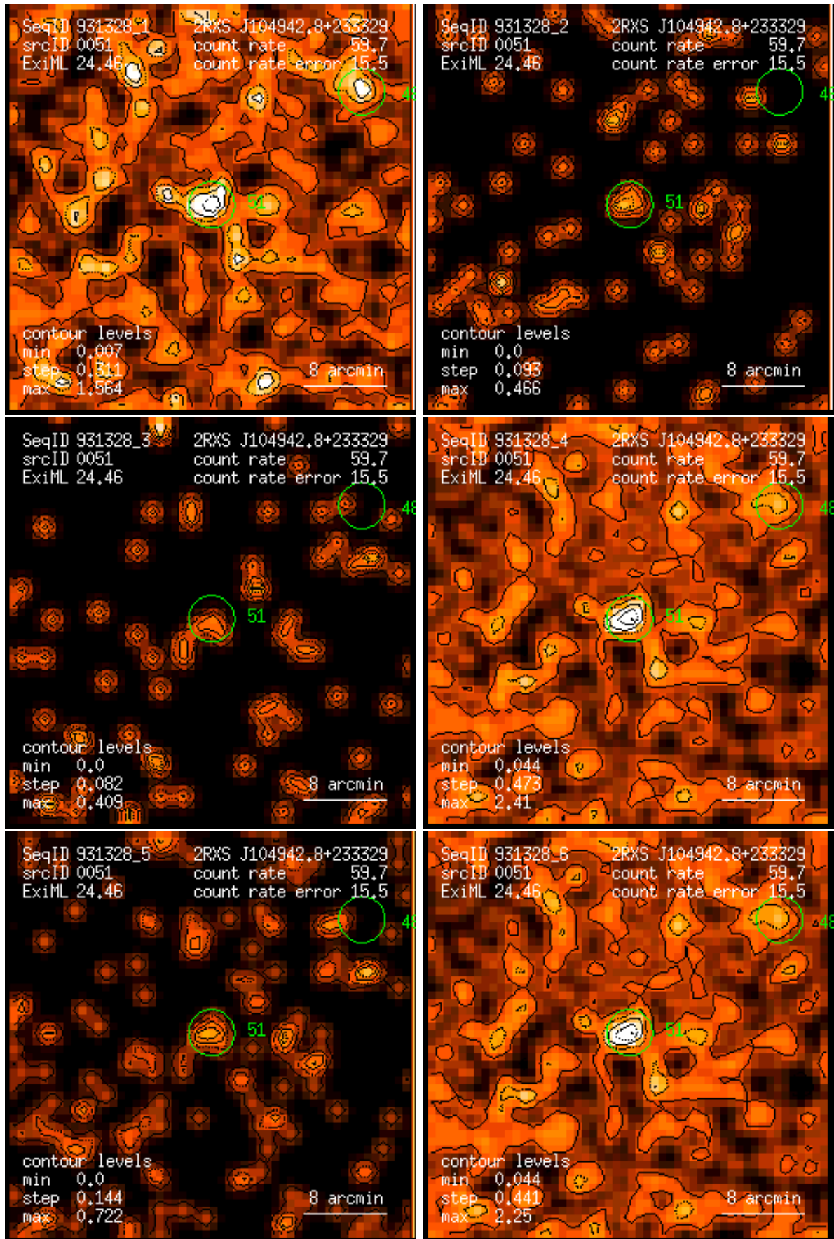
Figure 51: RASS 931328: detection 0051: band rate images, Gaussian filter: (1) PSPC channels 11 – 41, (2) 52 – 90, (3) 91 – 201, (4) 11 – 235, (5) 52 – 201, (6) 11 – 201. Broad band rates in counts/ks. Band rate contour levels in counts/ks/arcmin 2 .
