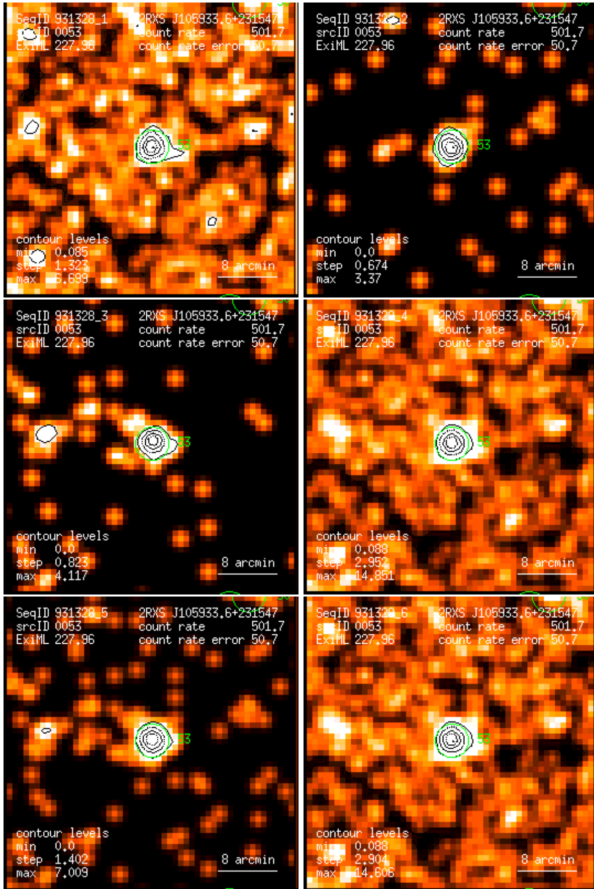
Figure 53: RASS 931328: detection 0053: band rate images, Gaussian filter: (1) PSPC channels 11 – 41, (2) 52 – 90, (3) 91 – 201, (4) 11 – 235, (5) 52 – 201, (6) 11 – 201. Broad band rates in counts/ks. Band rate contour levels in counts/ks/arcmin 2 .
