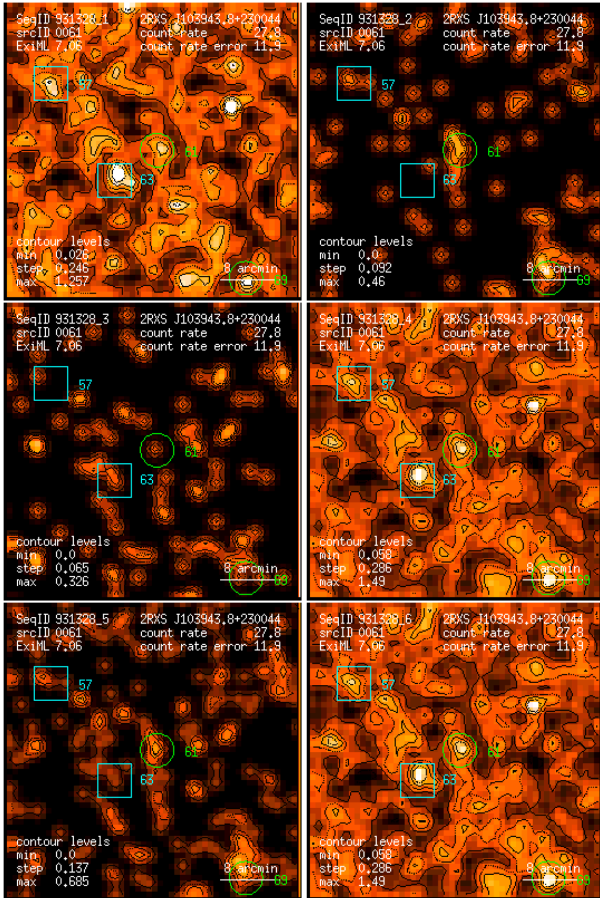
Figure 61: RASS 931328: detection 0061: band rate images, Gaussian filter: (1) PSPC channels 11 – 41, (2) 52 – 90, (3) 91 – 201, (4) 11 – 235, (5) 52 – 201, (6) 11 – 201. Broad band rates in counts/ks. Band rate contour levels in counts/ks/arcmin 2 .
