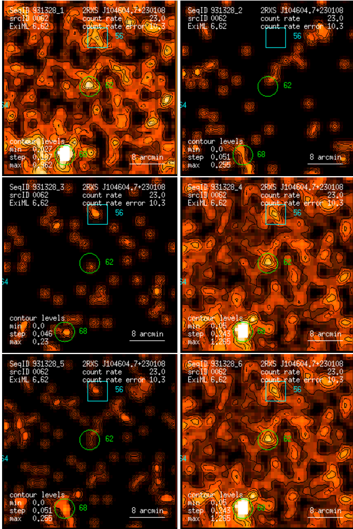
Figure 62: RASS 931328: detection 0062: band rate images, Gaussian filter: (1) PSPC channels 11 – 41, (2) 52 – 90, (3) 91 – 201, (4) 11 – 235, (5) 52 – 201, (6) 11 – 201. Broad band rates in counts/ks. Band rate contour levels in counts/ks/arcmin 2 .
