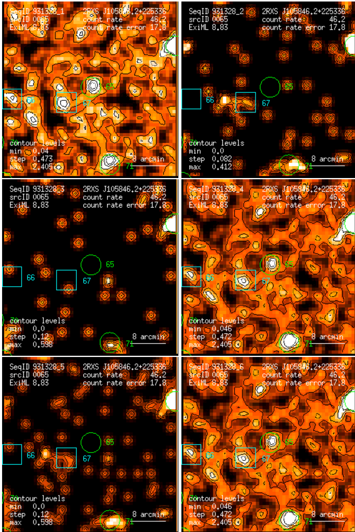
Figure 65: RASS 931328: detection 0065: band rate images, Gaussian filter: (1) PSPC channels 11 – 41, (2) 52 – 90, (3) 91 – 201, (4) 11 – 235, (5) 52 – 201, (6) 11 – 201. Broad band rates in counts/ks. Band rate contour levels in counts/ks/arcmin 2 .
