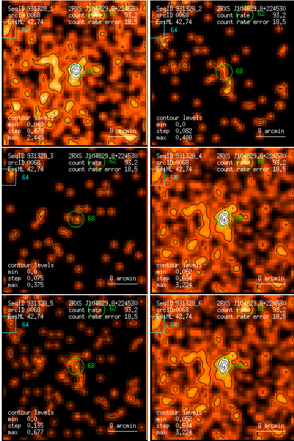
Figure 68: RASS 931328: detection 0068: band rate images, Gaussian filter: (1) PSPC channels 11 – 41, (2) 52 – 90, (3) 91 – 201, (4) 11 – 235, (5) 52 – 201, (6) 11 – 201. Broad band rates in counts/ks. Band rate contour levels in counts/ks/arcmin 2 .
