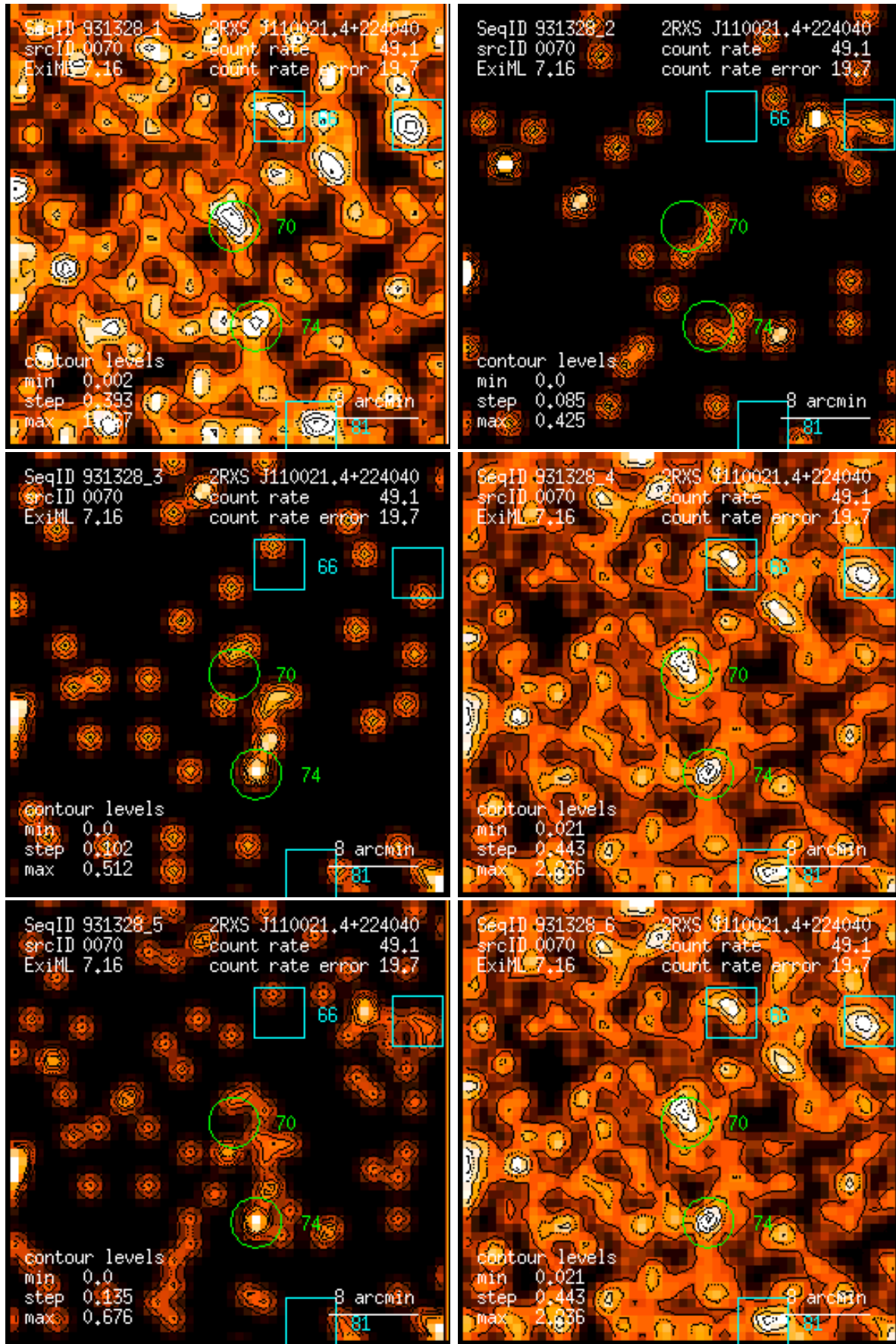
Figure 70: RASS 931328: detection 0070: band rate images, Gaussian filter: (1) PSPC channels 11 – 41, (2) 52 – 90, (3) 91 – 201, (4) 11 – 235, (5) 52 – 201, (6) 11 – 201. Broad band rates in counts/ks. Band rate contour levels in counts/ks/arcmin 2 .
