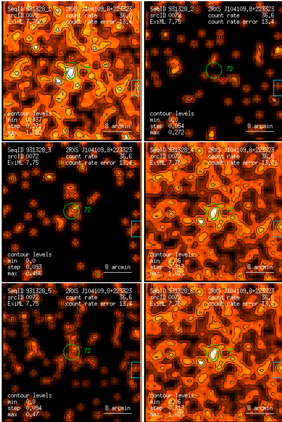
Figure 72: RASS 931328: detection 0072: band rate images, Gaussian filter: (1) PSPC channels 11 – 41, (2) 52 – 90, (3) 91 – 201, (4) 11 – 235, (5) 52 – 201, (6) 11 – 201. Broad band rates in counts/ks. Band rate contour levels in counts/ks/arcmin 2 .
