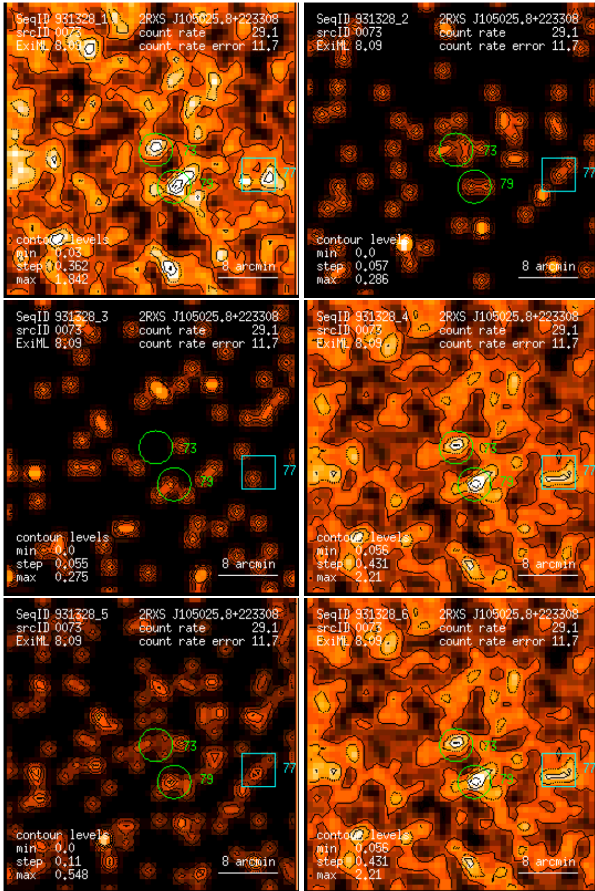
Figure 73: RASS 931328: detection 0073: band rate images, Gaussian filter: (1) PSPC channels 11 – 41, (2) 52 – 90, (3) 91 – 201, (4) 11 – 235, (5) 52 – 201, (6) 11 – 201. Broad band rates in counts/ks. Band rate contour levels in counts/ks/arcmin 2 .
