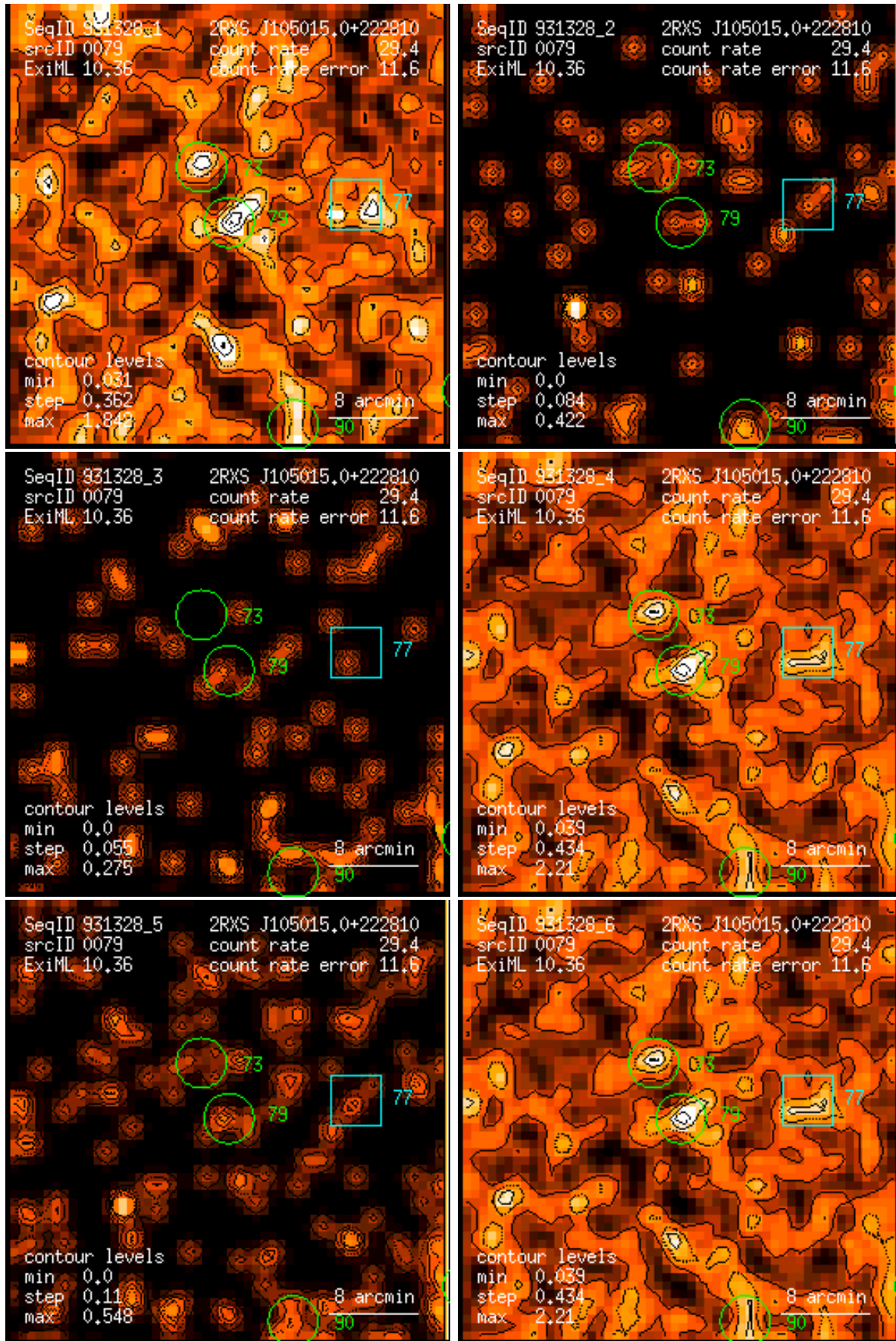
Figure 79: RASS 931328: detection 0079: band rate images, Gaussian filter: (1) PSPC channels 11 – 41, (2) 52 – 90, (3) 91 – 201, (4) 11 – 235, (5) 52 – 201, (6) 11 – 201. Broad band rates in counts/ks. Band rate contour levels in counts/ks/arcmin 2 .
