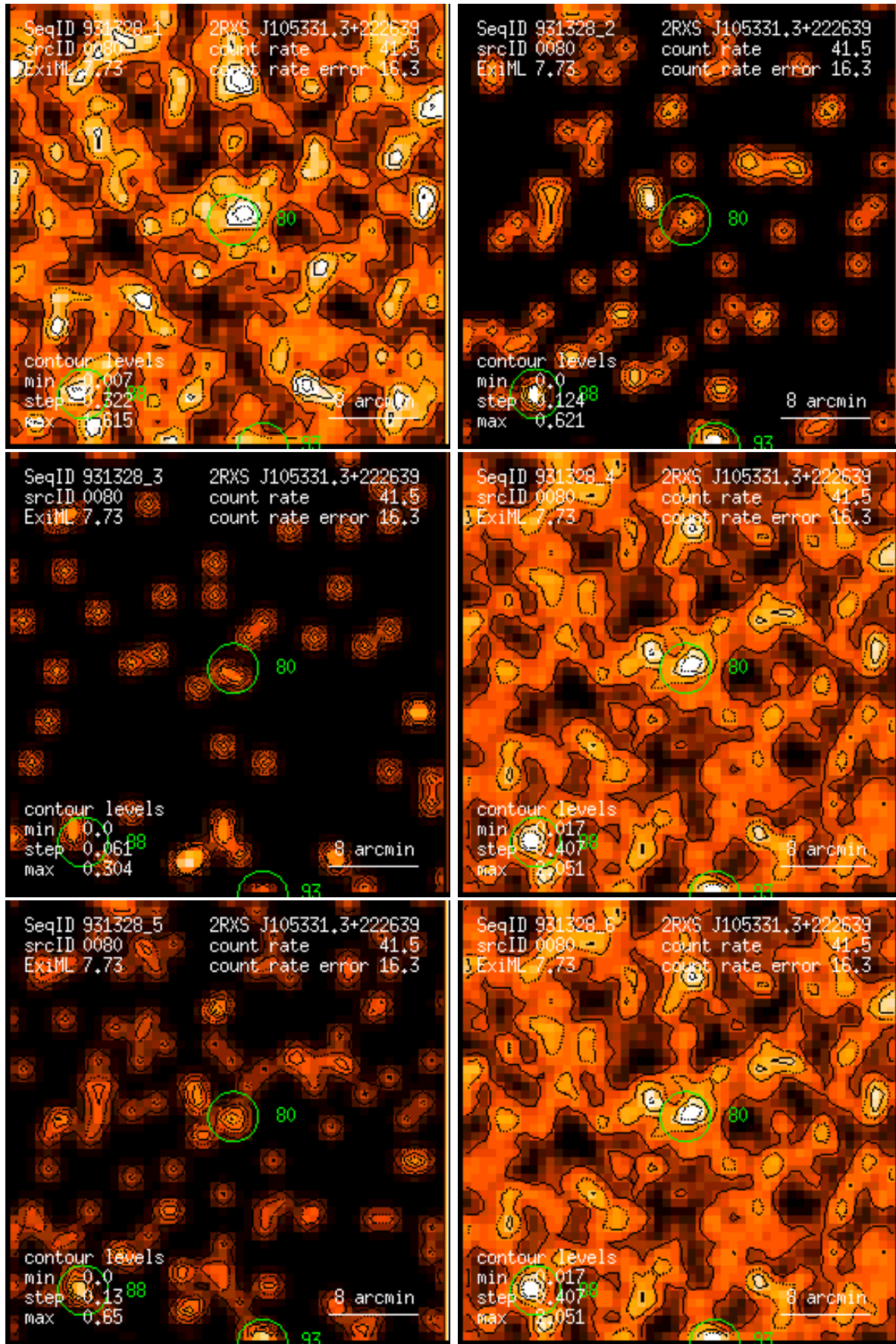
Figure 80: RASS 931328: detection 0080: band rate images, Gaussian filter: (1) PSPC channels 11 – 41, (2) 52 – 90, (3) 91 – 201, (4) 11 – 235, (5) 52 – 201, (6) 11 – 201. Broad band rates in counts/ks. Band rate contour levels in counts/ks/arcmin 2 .
