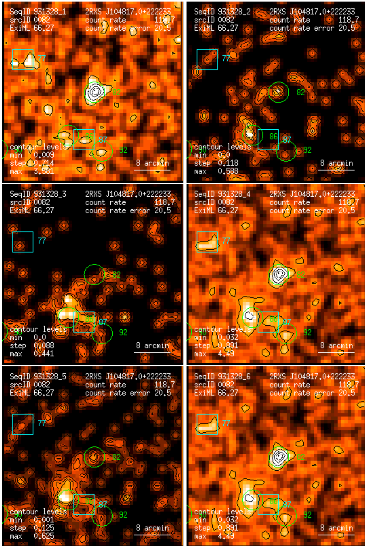
Figure 82: RASS 931328: detection 0082: band rate images, Gaussian filter: (1) PSPC channels 11 – 41, (2) 52 – 90, (3) 91 – 201, (4) 11 – 235, (5) 52 – 201, (6) 11 – 201. Broad band rates in counts/ks. Band rate contour levels in counts/ks/arcmin 2 .
