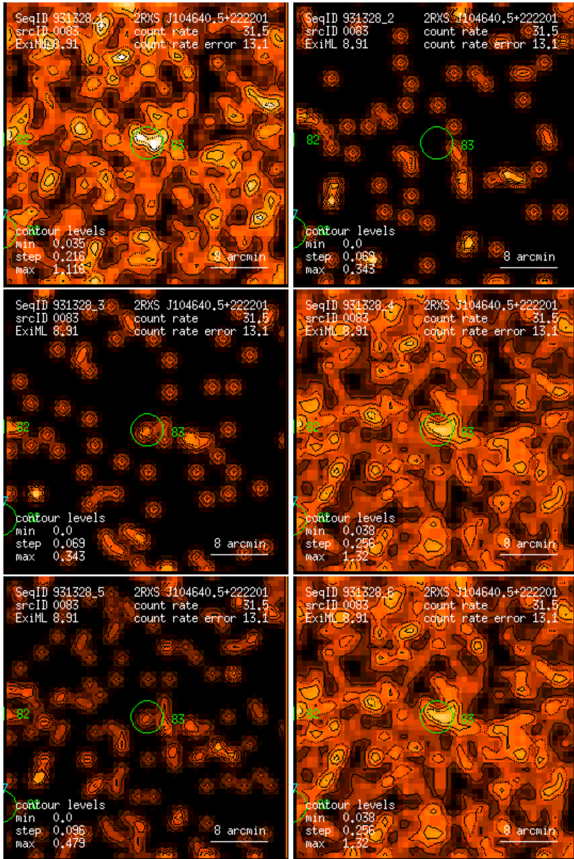
Figure 83: RASS 931328: detection 0083: band rate images, Gaussian filter: (1) PSPC channels 11 – 41, (2) 52 – 90, (3) 91 – 201, (4) 11 – 235, (5) 52 – 201, (6) 11 – 201. Broad band rates in counts/ks. Band rate contour levels in counts/ks/arcmin 2 .
