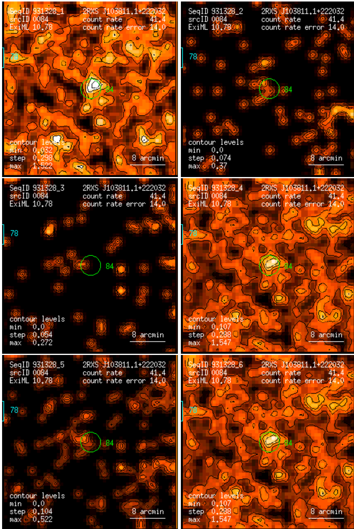
Figure 84: RASS 931328: detection 0084: band rate images, Gaussian filter: (1) PSPC channels 11 – 41, (2) 52 – 90, (3) 91 – 201, (4) 11 – 235, (5) 52 – 201, (6) 11 – 201. Broad band rates in counts/ks. Band rate contour levels in counts/ks/arcmin 2 .
