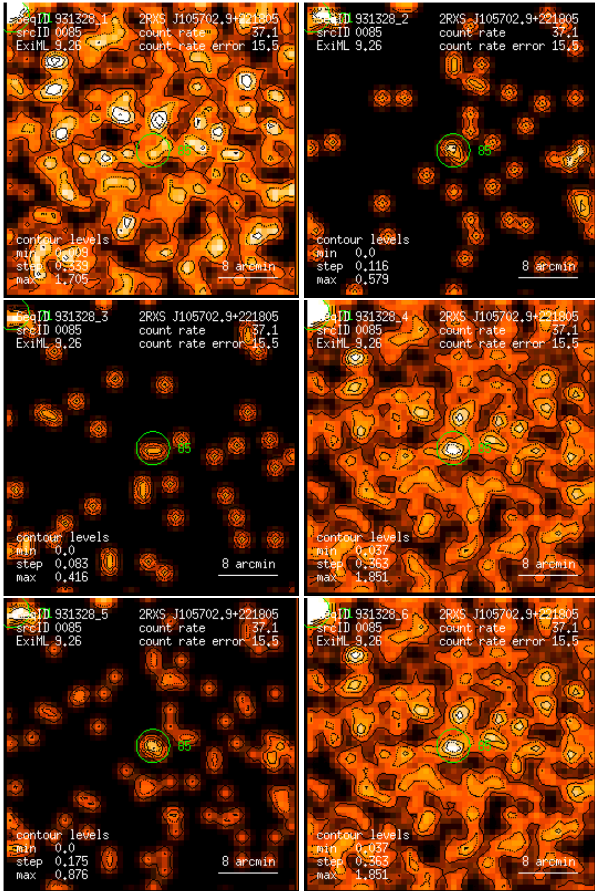
Figure 85: RASS 931328: detection 0085: band rate images, Gaussian filter: (1) PSPC channels 11 – 41, (2) 52 – 90, (3) 91 – 201, (4) 11 – 235, (5) 52 – 201, (6) 11 – 201. Broad band rates in counts/ks. Band rate contour levels in counts/ks/arcmin 2 .
