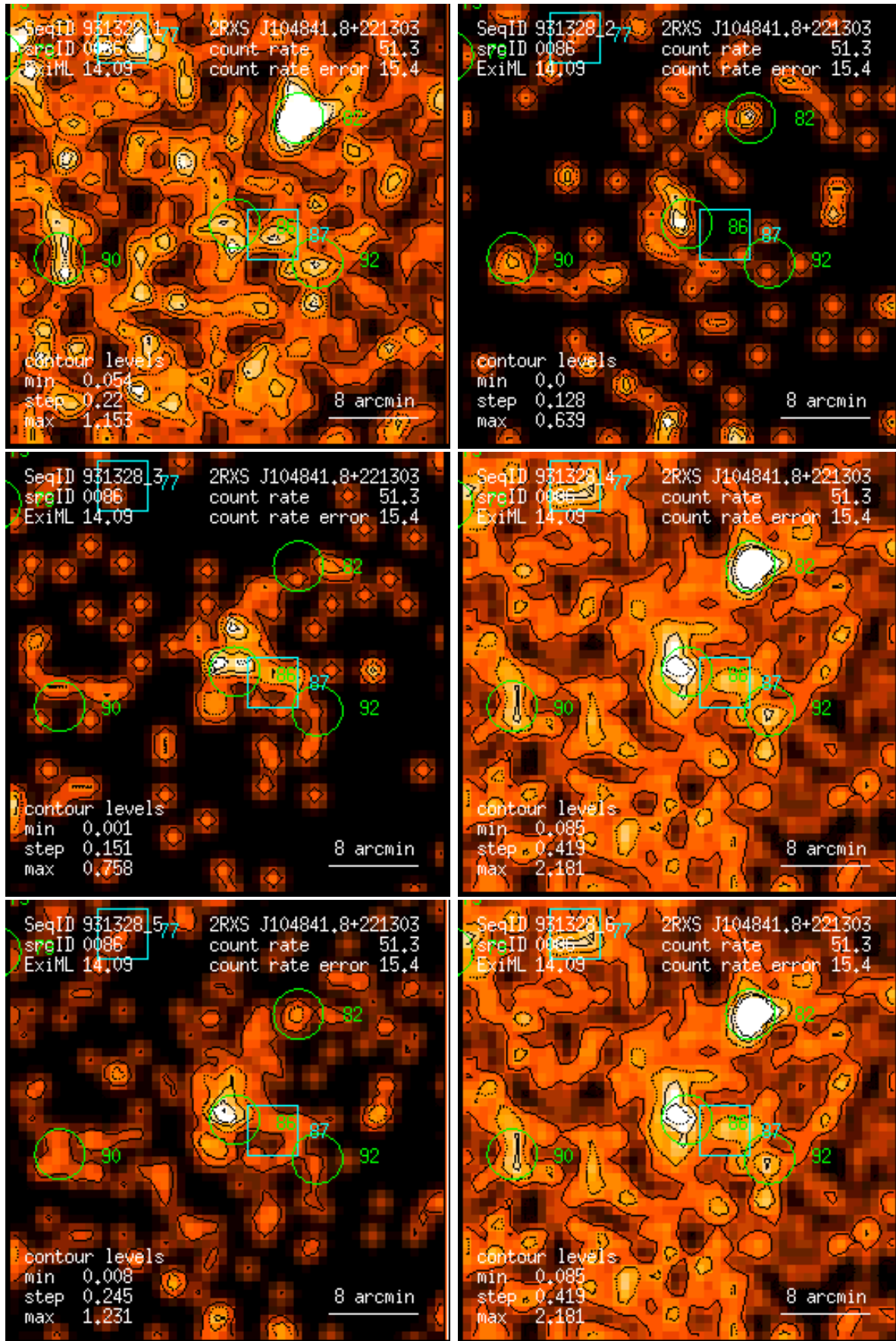
Figure 86: RASS 931328: detection 0086: band rate images, Gaussian filter: (1) PSPC channels 11 – 41, (2) 52 – 90, (3) 91 – 201, (4) 11 – 235, (5) 52 – 201, (6) 11 – 201. Broad band rates in counts/ks. Band rate contour levels in counts/ks/arcmin 2 .
