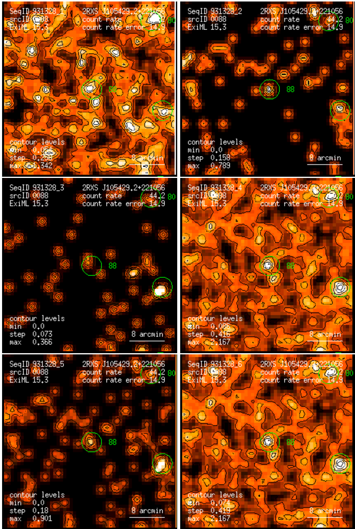
Figure 88: RASS 931328: detection 0088: band rate images, Gaussian filter: (1) PSPC channels 11 – 41, (2) 52 – 90, (3) 91 – 201, (4) 11 – 235, (5) 52 – 201, (6) 11 – 201. Broad band rates in counts/ks. Band rate contour levels in counts/ks/arcmin 2 .
