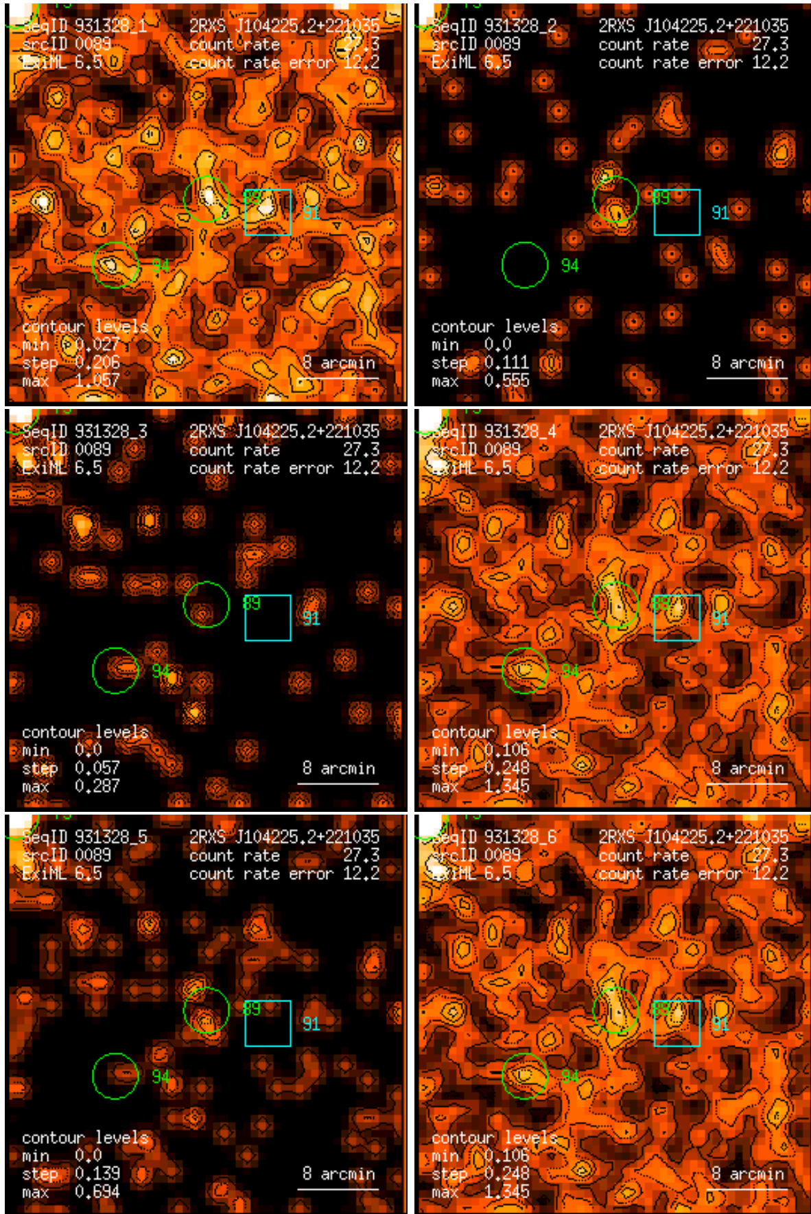
Figure 89: RASS 931328: detection 0089: band rate images, Gaussian filter: (1) PSPC channels 11 – 41, (2) 52 – 90, (3) 91 – 201, (4) 11 – 235, (5) 52 – 201, (6) 11 – 201. Broad band rates in counts/ks. Band rate contour levels in counts/ks/arcmin 2 .
