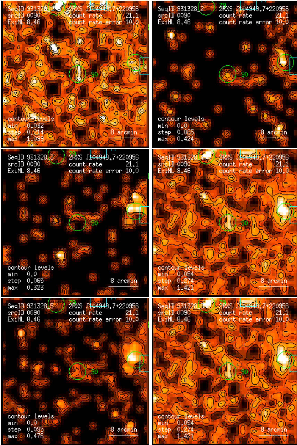
Figure 90: RASS 931328: detection 0090: band rate images, Gaussian filter: (1) PSPC channels 11 – 41, (2) 52 – 90, (3) 91 – 201, (4) 11 – 235, (5) 52 – 201, (6) 11 – 201. Broad band rates in counts/ks. Band rate contour levels in counts/ks/arcmin 2 .
