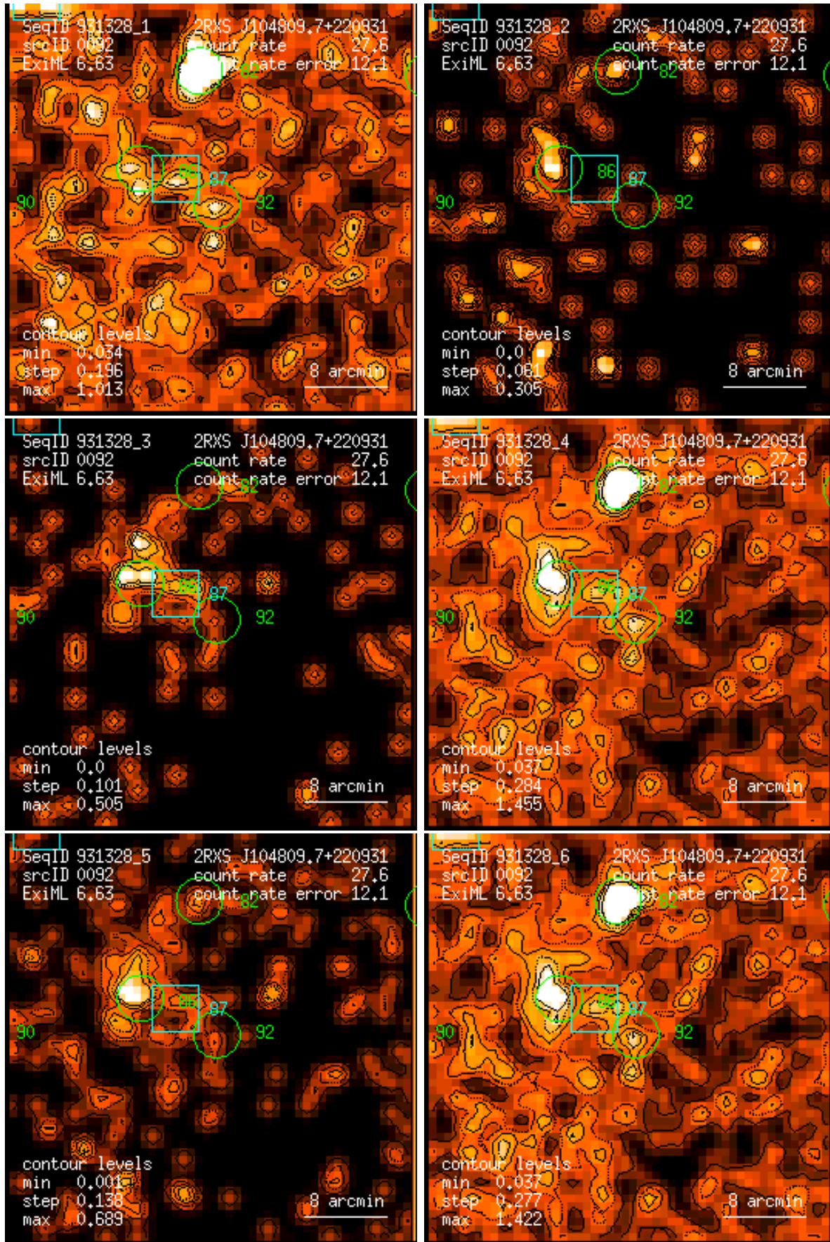
Figure 92: RASS 931328: detection 0092: band rate images, Gaussian filter: (1) PSPC channels 11 – 41, (2) 52 – 90, (3) 91 – 201, (4) 11 – 235, (5) 52 – 201, (6) 11 – 201. Broad band rates in counts/ks. Band rate contour levels in counts/ks/arcmin 2 .
