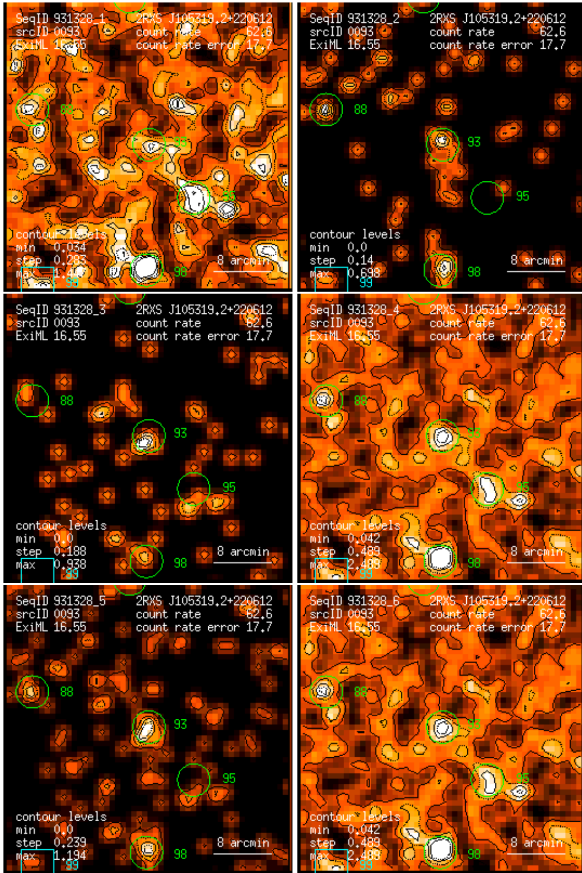
Figure 93: RASS 931328: detection 0093: band rate images, Gaussian filter: (1) PSPC channels 11 – 41, (2) 52 – 90, (3) 91 – 201, (4) 11 – 235, (5) 52 – 201, (6) 11 – 201. Broad band rates in counts/ks. Band rate contour levels in counts/ks/arcmin 2 .
