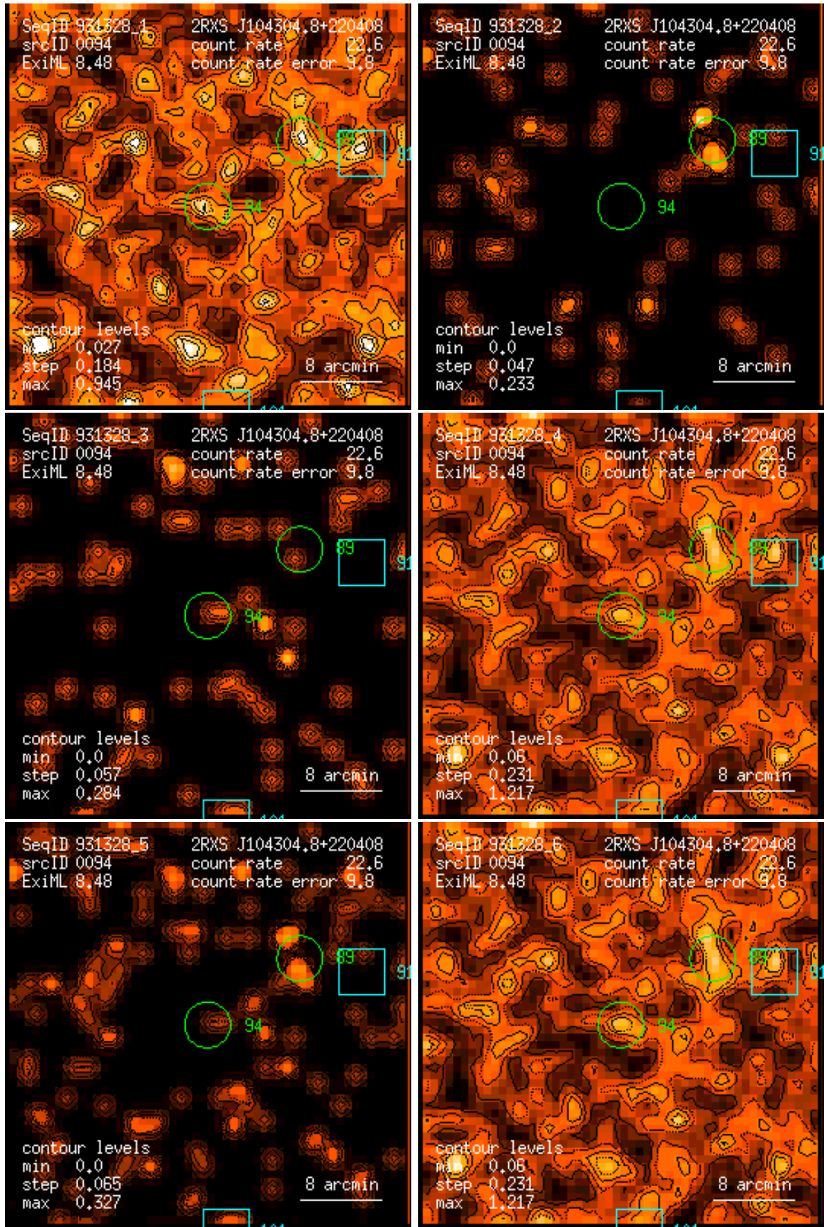
Figure 94: RASS 931328: detection 0094: band rate images, Gaussian filter: (1) PSPC channels 11 – 41, (2) 52 – 90, (3) 91 – 201, (4) 11 – 235, (5) 52 – 201, (6) 11 – 201. Broad band rates in counts/ks. Band rate contour levels in counts/ks/arcmin 2 .
