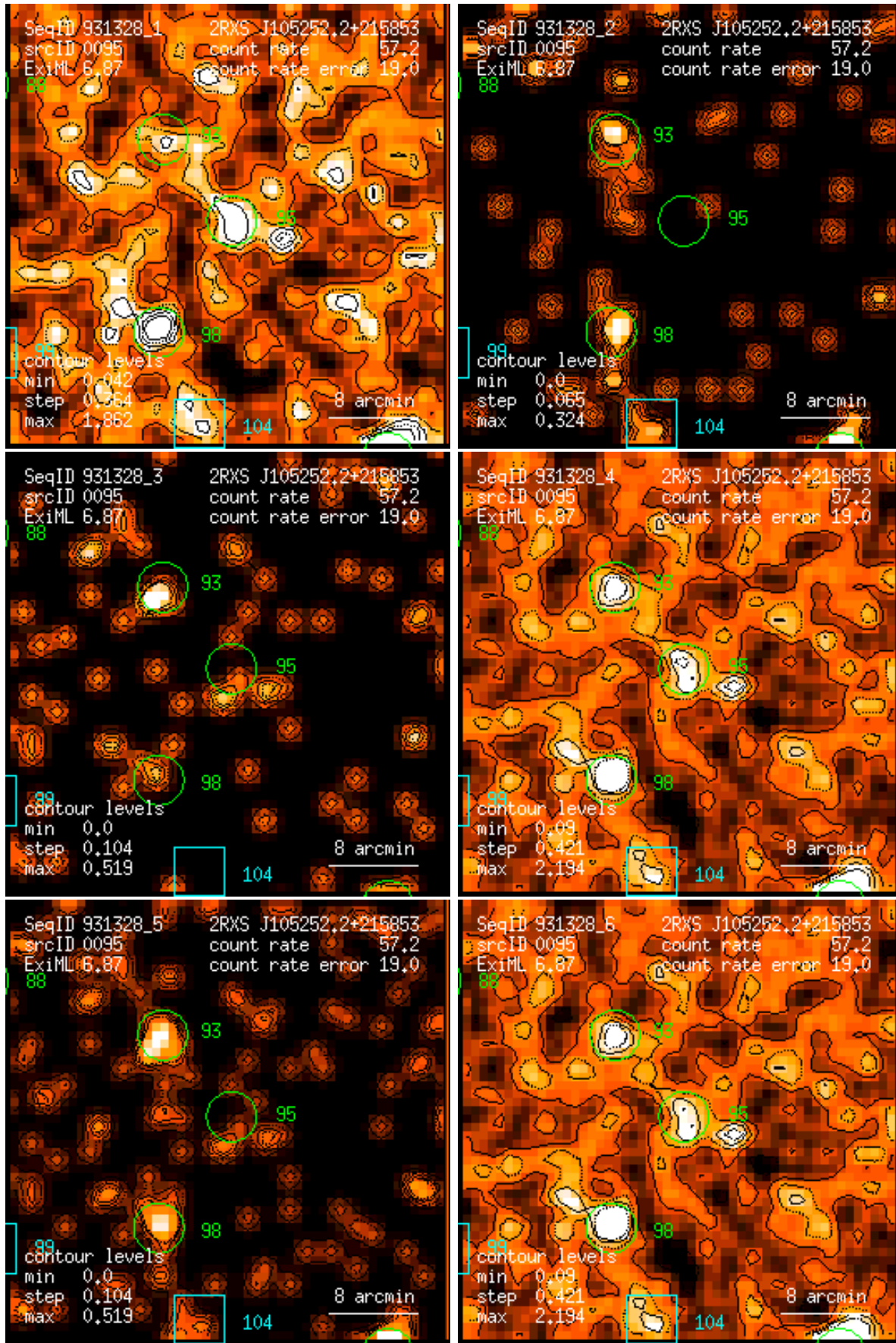
Figure 95: RASS 931328: detection 0095: band rate images, Gaussian filter: (1) PSPC channels 11 – 41, (2) 52 – 90, (3) 91 – 201, (4) 11 – 235, (5) 52 – 201, (6) 11 – 201. Broad band rates in counts/ks. Band rate contour levels in counts/ks/arcmin 2 .
