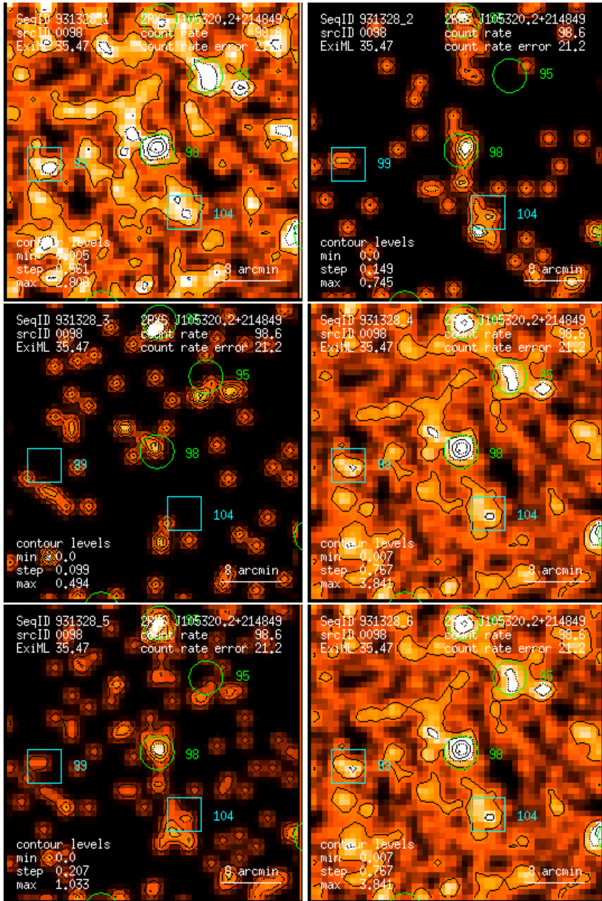
Figure 98: RASS 931328: detection 0098: band rate images, Gaussian filter: (1) PSPC channels 11 – 41, (2) 52 – 90, (3) 91 – 201, (4) 11 – 235, (5) 52 – 201, (6) 11 – 201. Broad band rates in counts/ks. Band rate contour levels in counts/ks/arcmin 2 .
