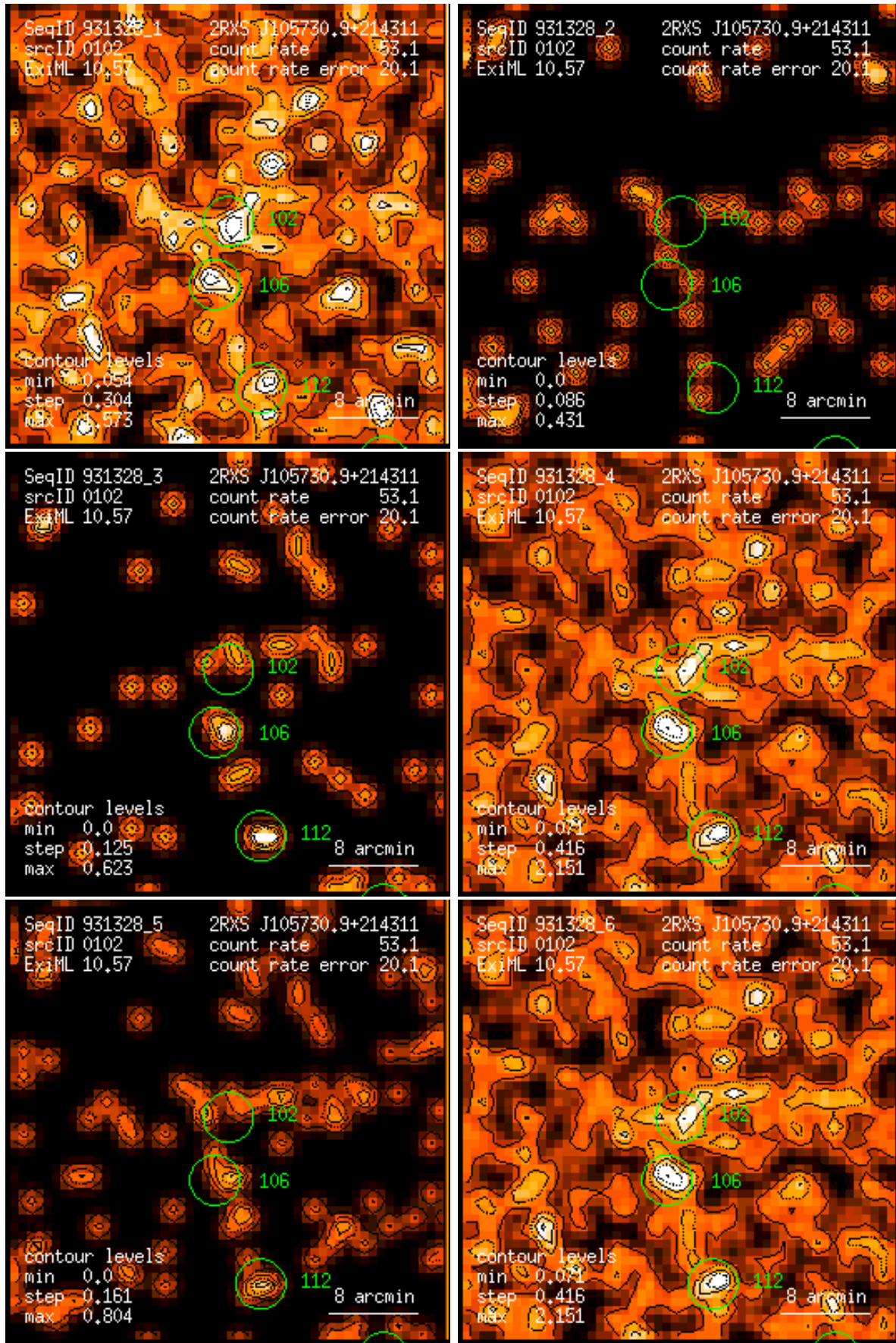
Figure 102: RASS 931328: detection 0102: band rate images, Gaussian filter: (1) PSPC channels 11 – 41, (2) 52 – 90, (3) 91 – 201, (4) 11 – 235, (5) 52 – 201, (6) 11 – 201. Broad band rates in counts/ks. Band rate contour levels in counts/ks/arcmin 2 .
