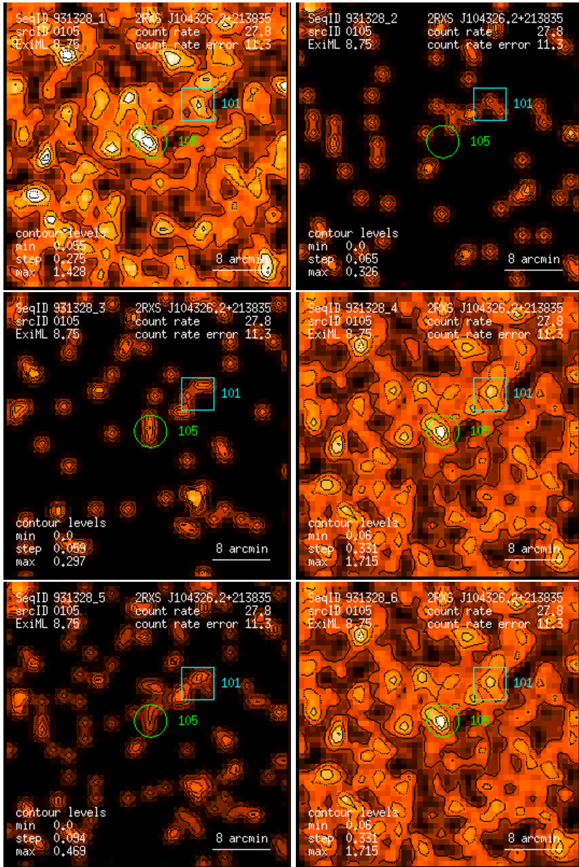
Figure 105: RASS 931328: detection 0105: band rate images, Gaussian filter: (1) PSPC channels 11 – 41, (2) 52 – 90, (3) 91 – 201, (4) 11 – 235, (5) 52 – 201, (6) 11 – 201. Broad band rates in counts/ks. Band rate contour levels in counts/ks/arcmin 2 .
