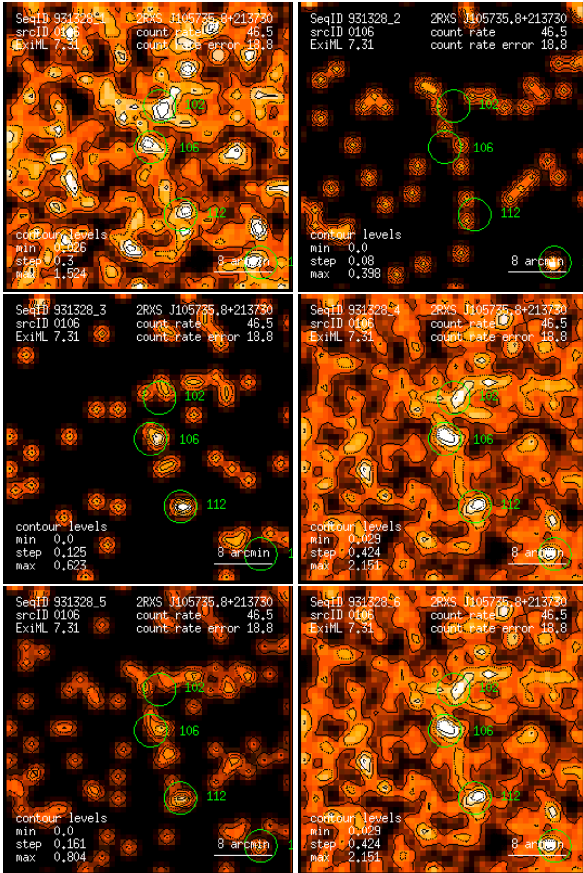
Figure 106: RASS 931328: detection 0106: band rate images, Gaussian filter: (1) PSPC channels 11 – 41, (2) 52 – 90, (3) 91 – 201, (4) 11 – 235, (5) 52 – 201, (6) 11 – 201. Broad band rates in counts/ks. Band rate contour levels in counts/ks/arcmin 2 .
