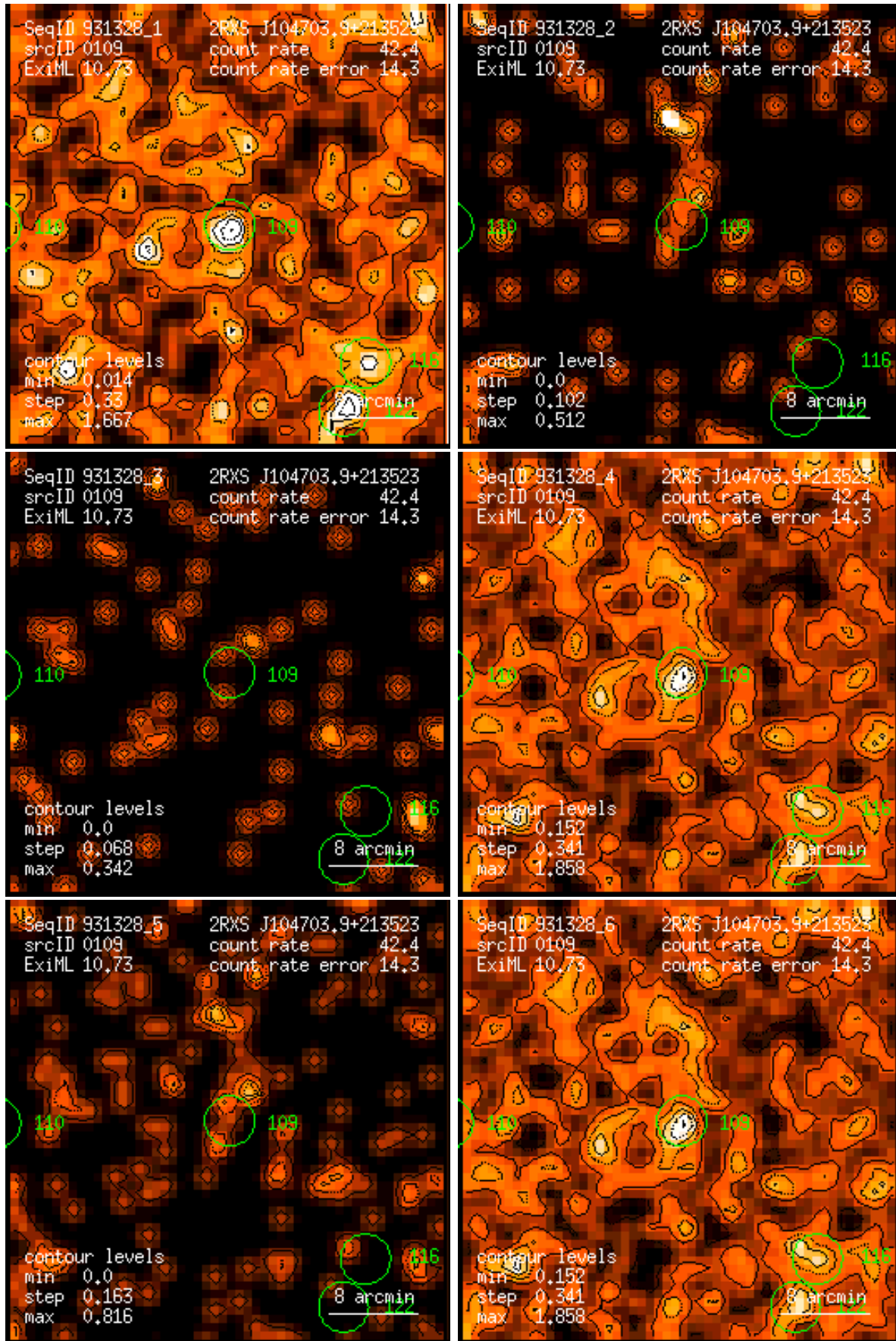
Figure 109: RASS 931328: detection 0109: band rate images, Gaussian filter: (1) PSPC channels 11 – 41, (2) 52 – 90, (3) 91 – 201, (4) 11 – 235, (5) 52 – 201, (6) 11 – 201. Broad band rates in counts/ks. Band rate contour levels in counts/ks/arcmin 2 .
