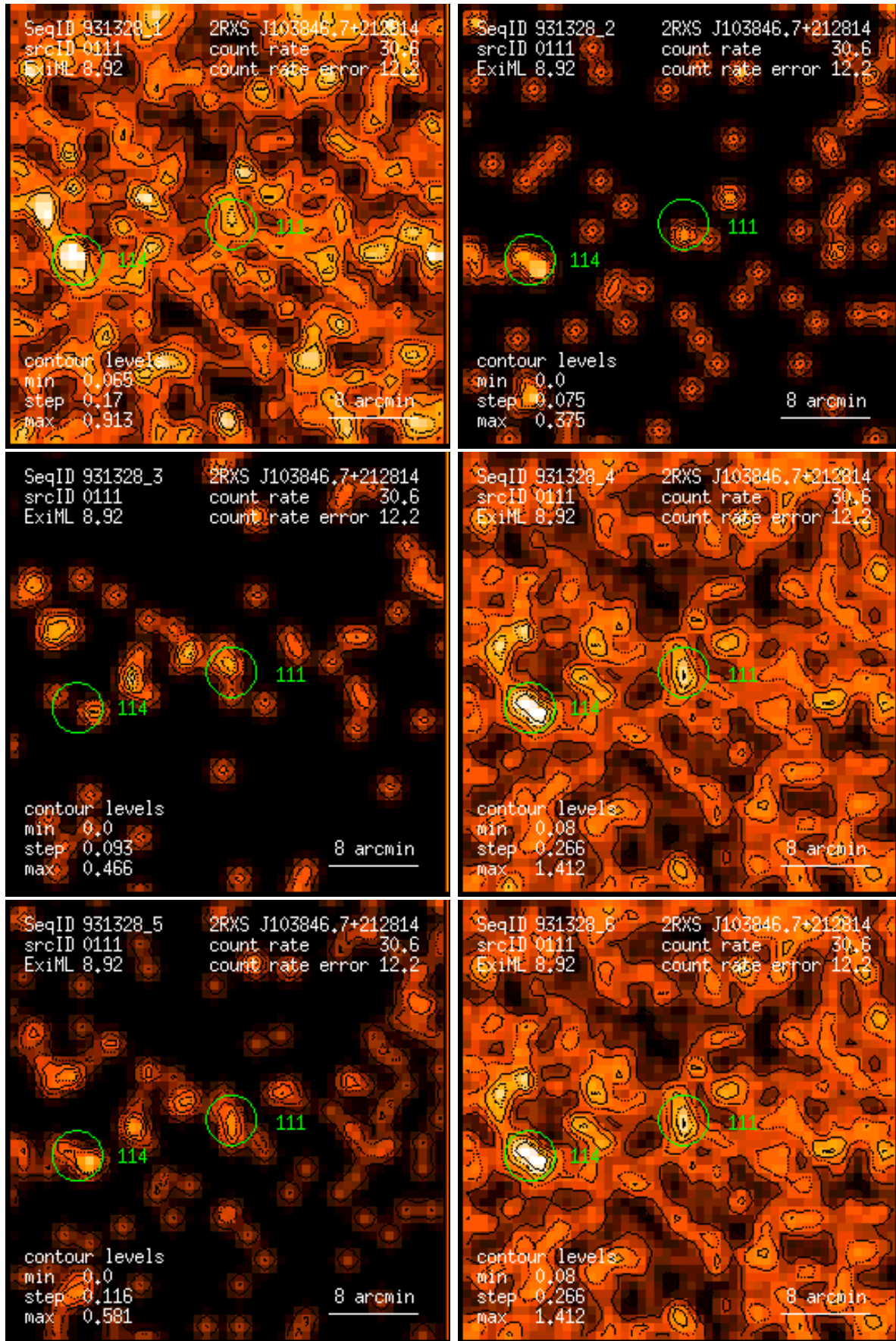
Figure 111: RASS 931328: detection 0111: band rate images, Gaussian filter: (1) PSPPC channels 11 – 41, (2) 52 – 90, (3) 91 – 201, (4) 11 – 235, (5) 52 – 201, (6) 11 – 201. Broad band rates in counts/ks. Band rate contour levels in counts/ks/arcmin 2 .
