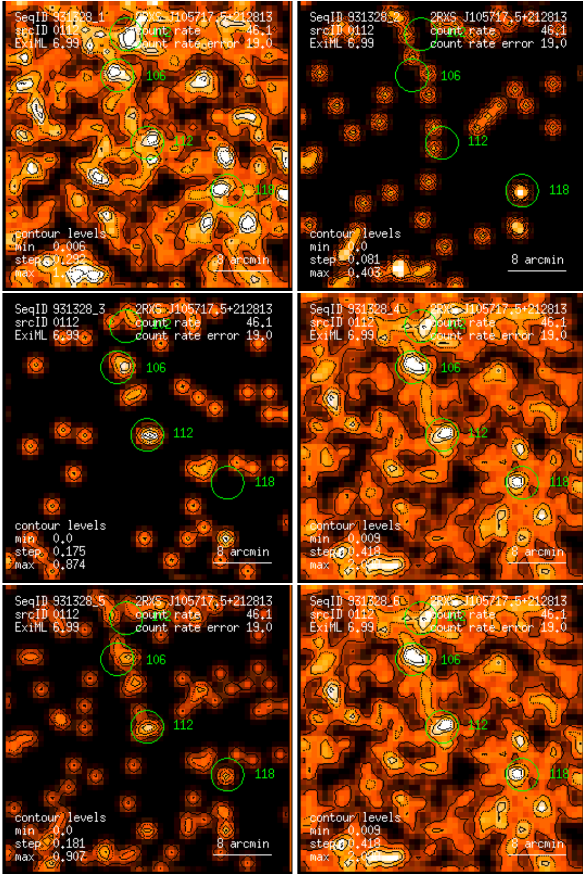
Figure 112: RASS 931328: detection 0112: band rate images, Gaussian filter: (1) PSPC channels 11 – 41, (2) 52 – 90, (3) 91 – 201, (4) 11 – 235, (5) 52 – 201, (6) 11 – 201. Broad band rates in counts/ks. Band rate contour levels in counts/ks/arcmin 2 .
