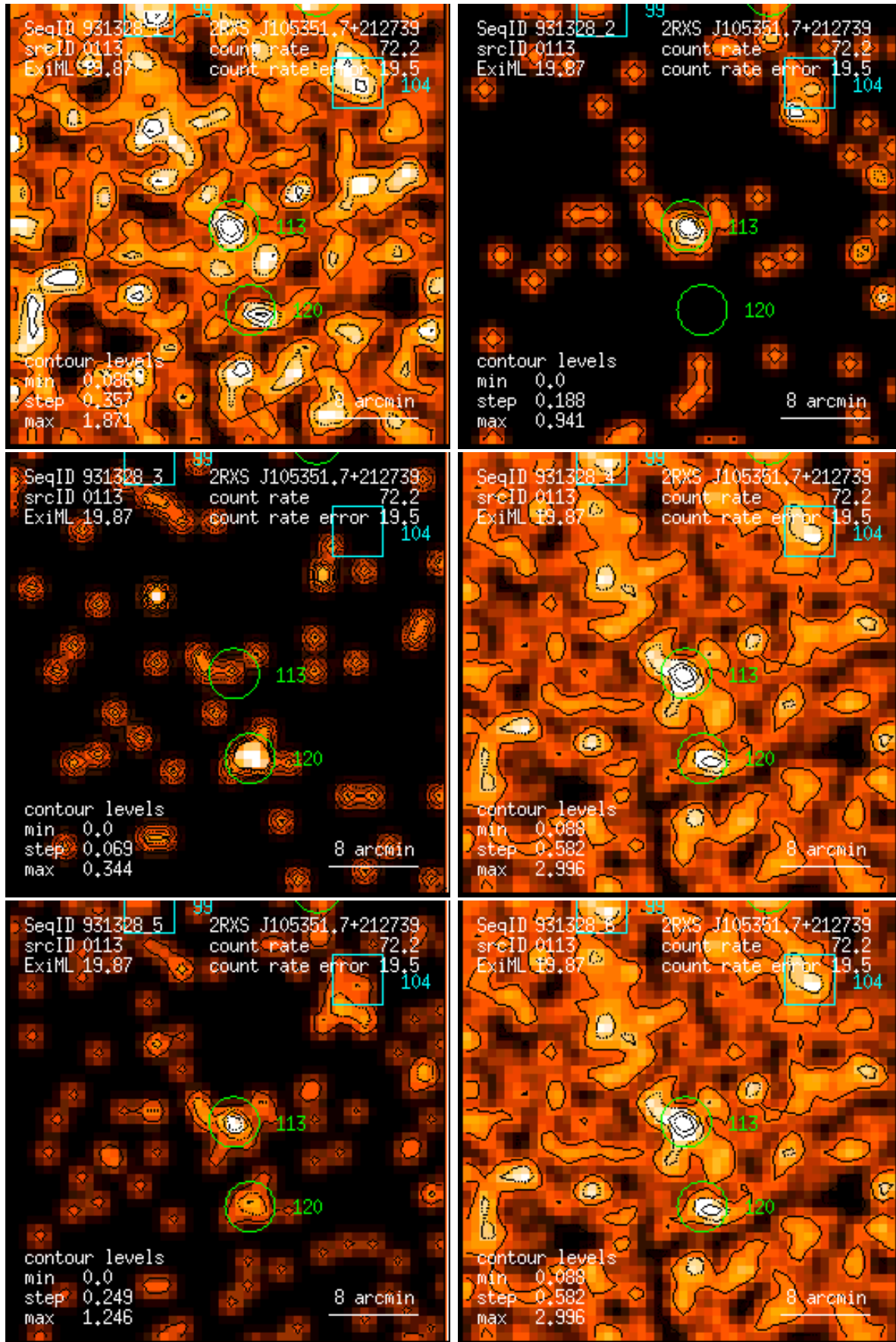
Figure 113: RASS 931328: detection 0113: band rate images, Gaussian filter: (1) PSPC channels 11 – 41, (2) 52 – 90, (3) 91 – 201, (4) 11 – 235, (5) 52 – 201, (6) 11 – 201. Broad band rates in counts/ks. Band rate contour levels in counts/ks/arcmin 2 .
