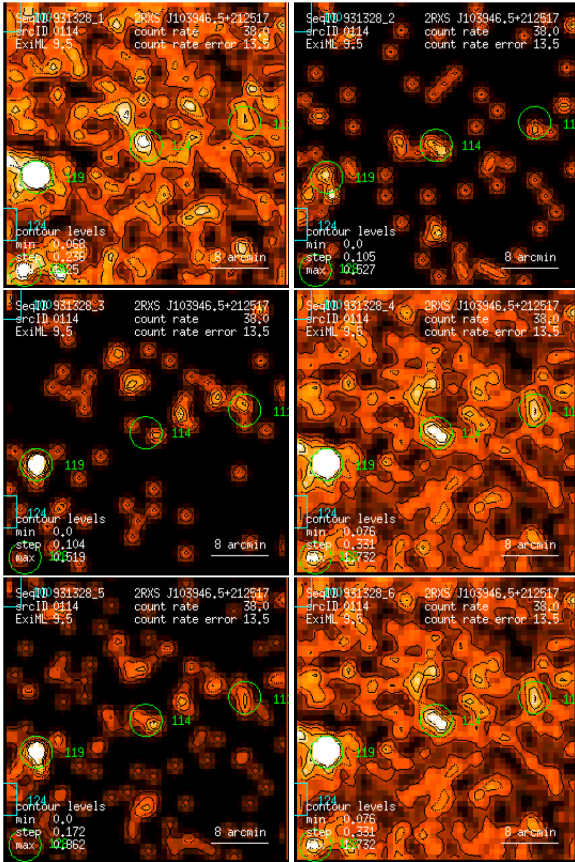
Figure 114: RASS 931328: detection 0114: band rate images, Gaussian filter: (1) PSPC channels 11 – 41, (2) 52 – 90, (3) 91 – 201, (4) 11 – 235, (5) 52 – 201, (6) 11 – 201. Broad band rates in counts/ks. Band rate contour levels in counts/ks/arcmin 2 .
