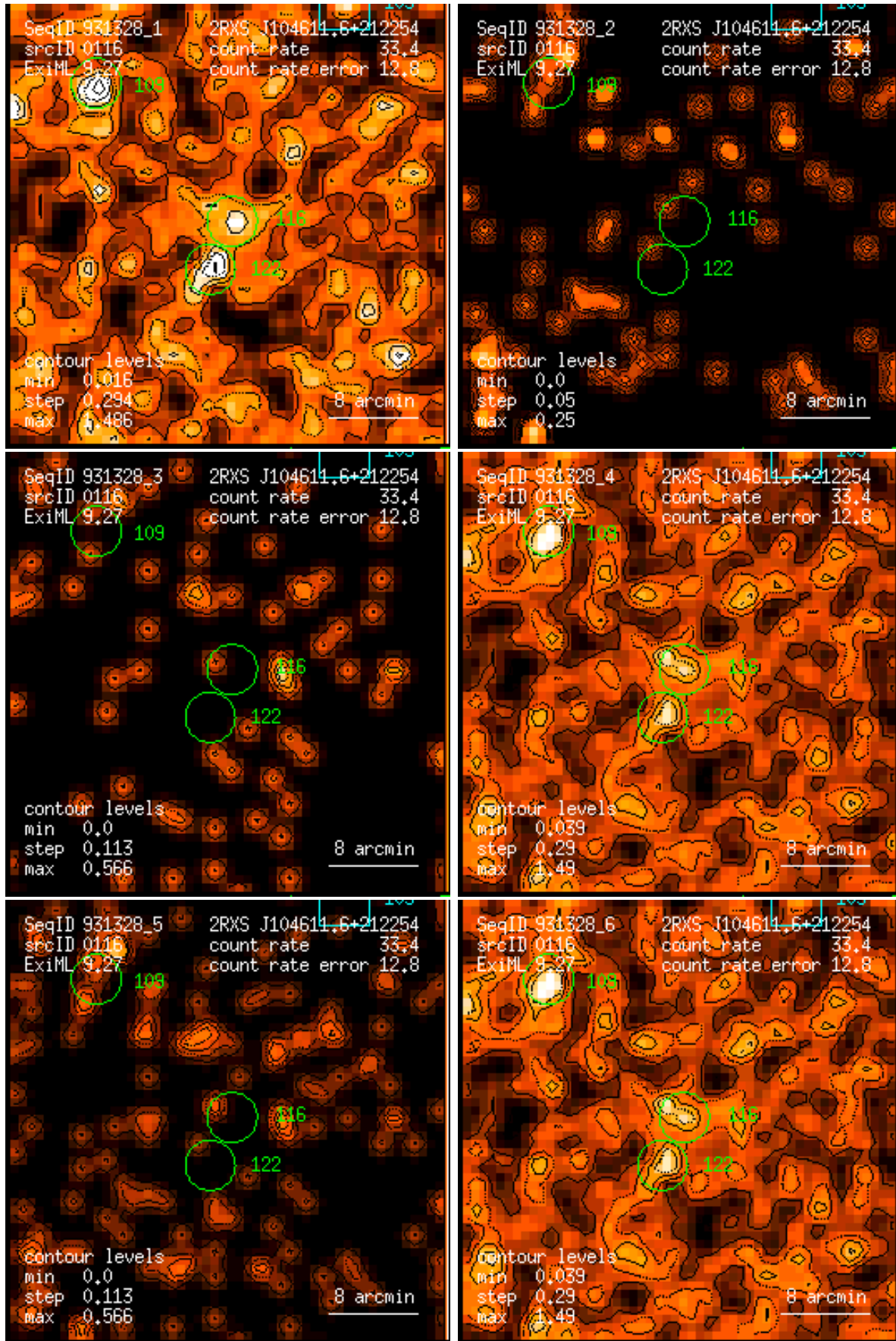
Figure 116: RASS 931328: detection 0116: band rate images, Gaussian filter: (1) PSPC channels 11 – 41, (2) 52 – 90, (3) 91 – 201, (4) 11 – 235, (5) 52 – 201, (6) 11 – 201. Broad band rates in counts/ks. Band rate contour levels in counts/ks/arcmin 2 .
