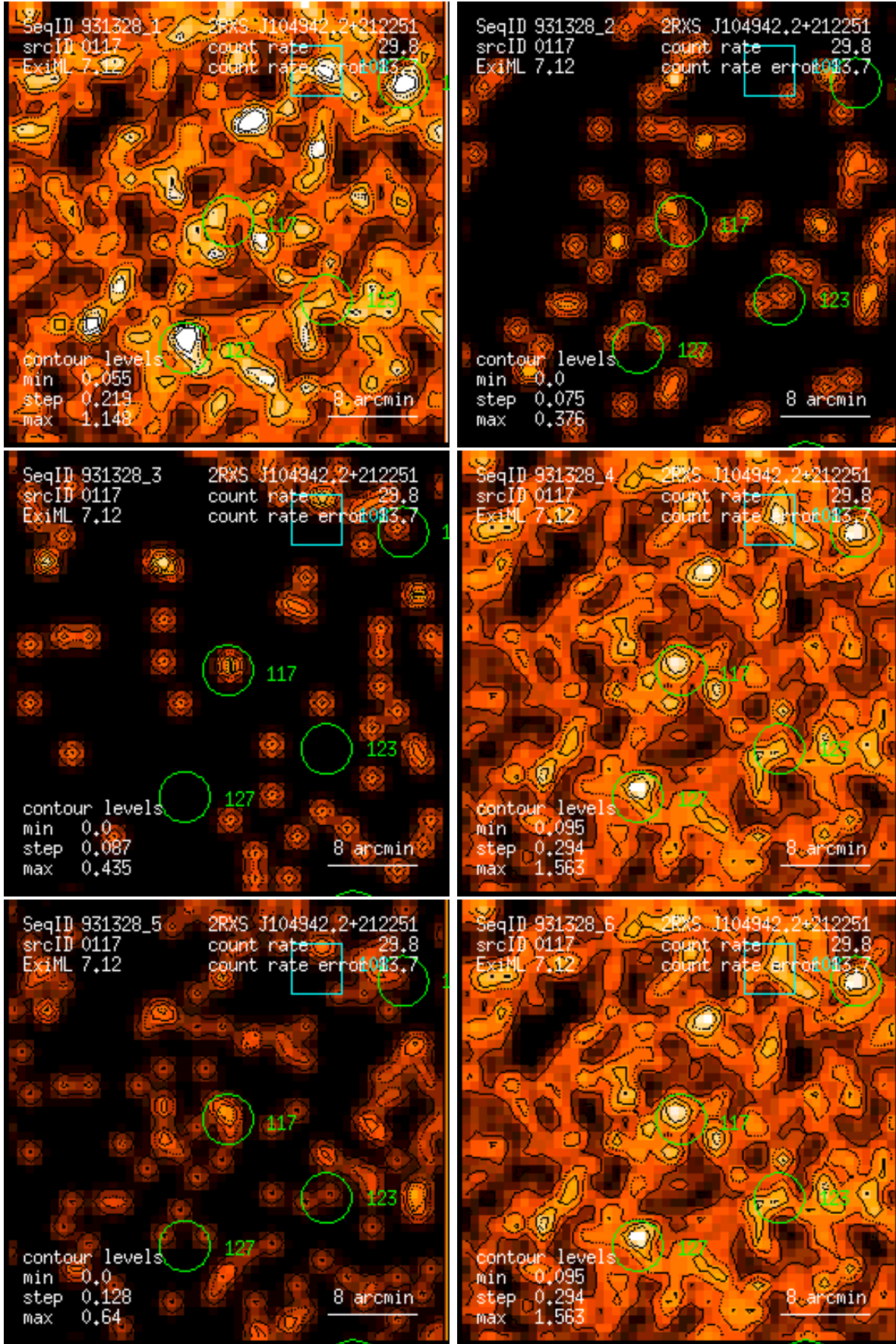
Figure 117: RASS 931328: detection 0117: band rate images, Gaussian filter: (1) PSPC channels 11 – 41, (2) 52 – 90, (3) 91 – 201, (4) 11 – 235, (5) 52 – 201, (6) 11 – 201. Broad band rates in counts/ks. Band rate contour levels in counts/ks/arcmin 2 .
