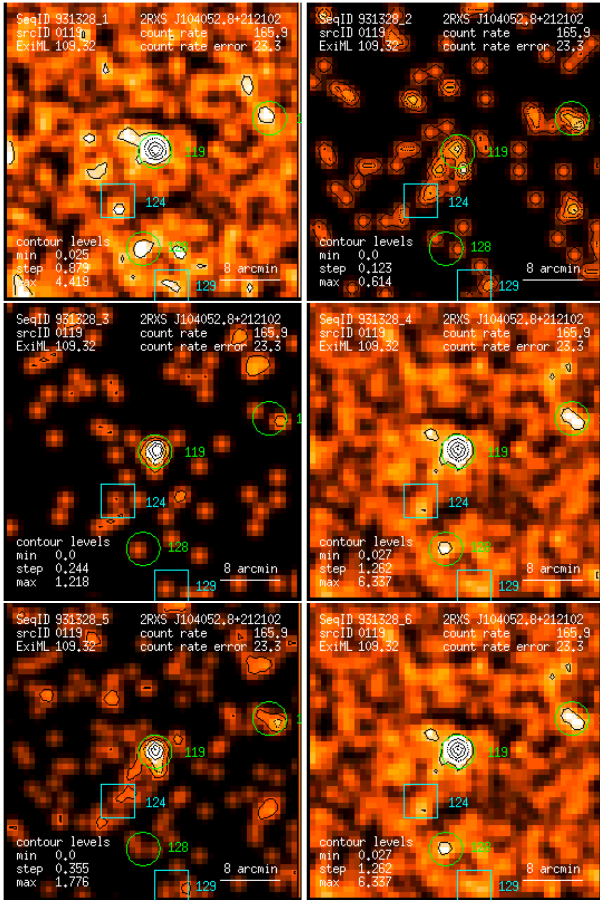
Figure 119: RASS 931328: detection 0119: band rate images, Gaussian filter: (1) PSPC channels 11 – 41, (2) 52 – 90, (3) 91 – 201, (4) 11 – 235, (5) 52 – 201, (6) 11 – 201. Broad band rates in counts/ks. Band rate contour levels in counts/ks/arcmin 2 .
