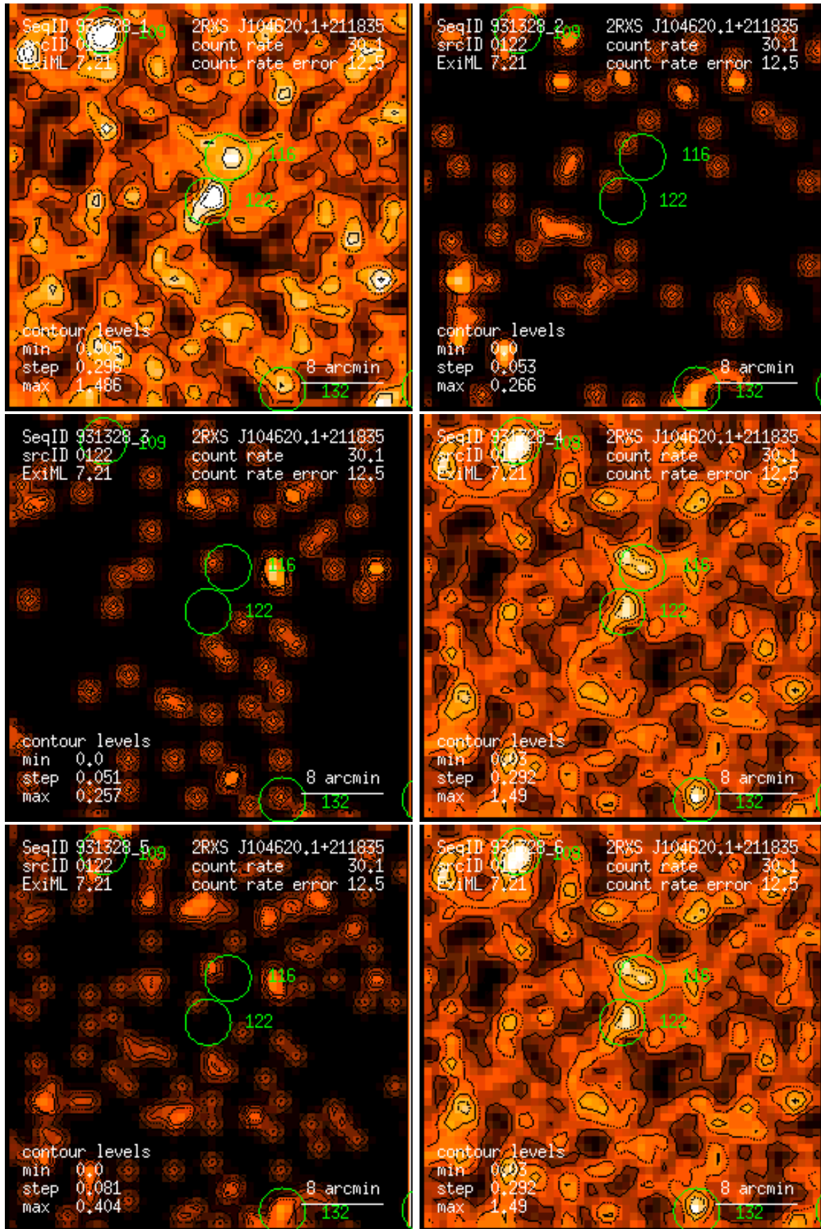
Figure 122: RASS 931328: detection 0122: band rate images, Gaussian filter: (1) PSPC channels 11 – 41, (2) 52 – 90, (3) 91 – 201, (4) 11 – 235, (5) 52 – 201, (6) 11 – 201. Broad band rates in counts/ks. Band rate contour levels in counts/ks/arcmin 2 .
