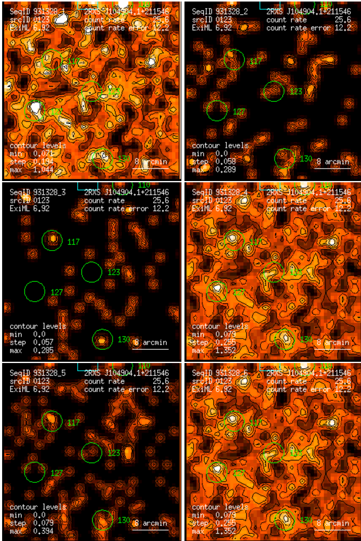
Figure 123: RASS 931328: detection 0123: band rate images, Gaussian filter: (1) PSPC channels 11 – 41, (2) 52 – 90, (3) 91 – 201, (4) 11 – 235, (5) 52 – 201, (6) 11 – 201. Broad band rates in counts/ks. Band rate contour levels in counts/ks/arcmin 2 .
