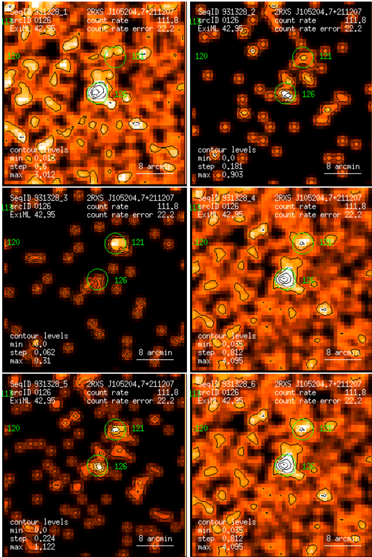
Figure 126: RASS 931328: detection 0126: band rate images, Gaussian filter: (1) PSPC channels 11 – 41, (2) 52 – 90, (3) 91 – 201, (4) 11 – 235, (5) 52 – 201, (6) 11 – 201. Broad band rates in counts/ks. Band rate contour levels in counts/ks/arcmin 2 .
