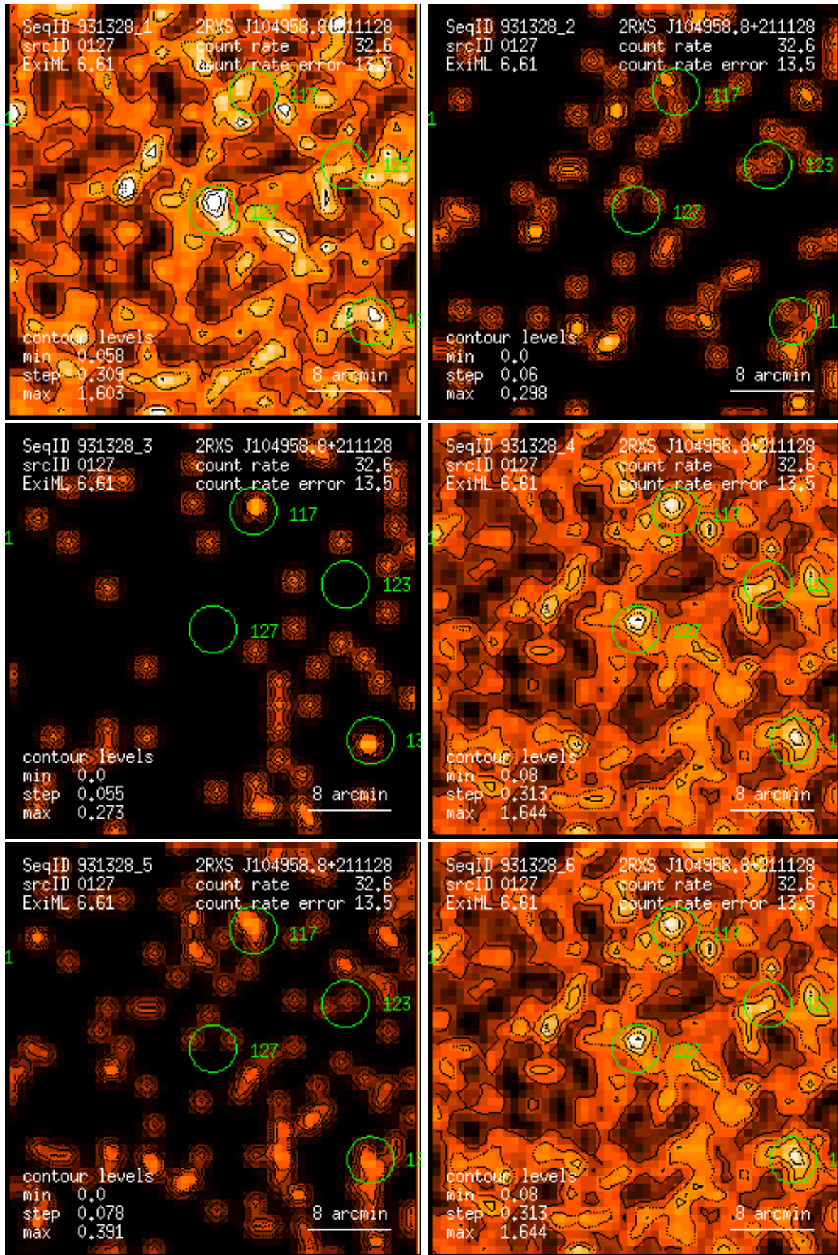
Figure 127: RASS 931328: detection 0127: band rate images, Gaussian filter: (1) PSPC channels 11 – 41, (2) 52 – 90, (3) 91 – 201, (4) 11 – 235, (5) 52 – 201, (6) 11 – 201. Broad band rates in counts/ks. Band rate contour levels in counts/ks/arcmin 2 .
