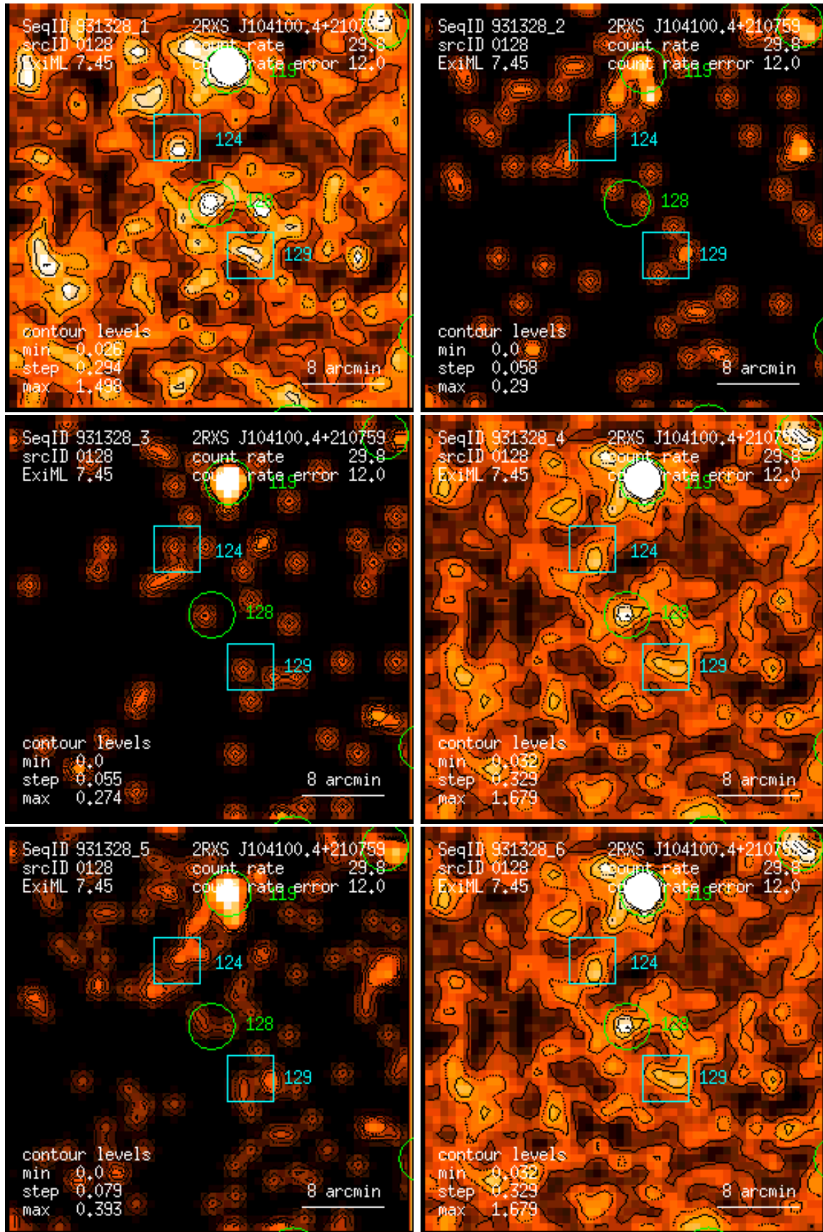
Figure 128: RASS 931328: detection 0128: band rate images, Gaussian filter: (1) PSPC channels 11 – 41, (2) 52 – 90, (3) 91 – 201, (4) 11 – 235, (5) 52 – 201, (6) 11 – 201. Broad band rates in counts/ks. Band rate contour levels in counts/ks/arcmin 2 .
