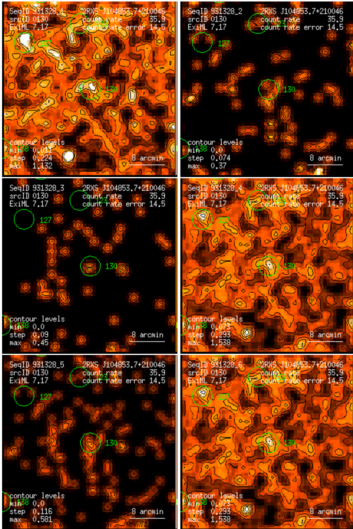
Figure 130: RASS 931328: detection 0130: band rate images, Gaussian filter: (1) PSPC channels 11 – 41, (2) 52 – 90, (3) 91 – 201, (4) 11 – 235, (5) 52 – 201, (6) 11 – 201. Broad band rates in counts/ks. Band rate contour levels in counts/ks/arcmin 2 .
