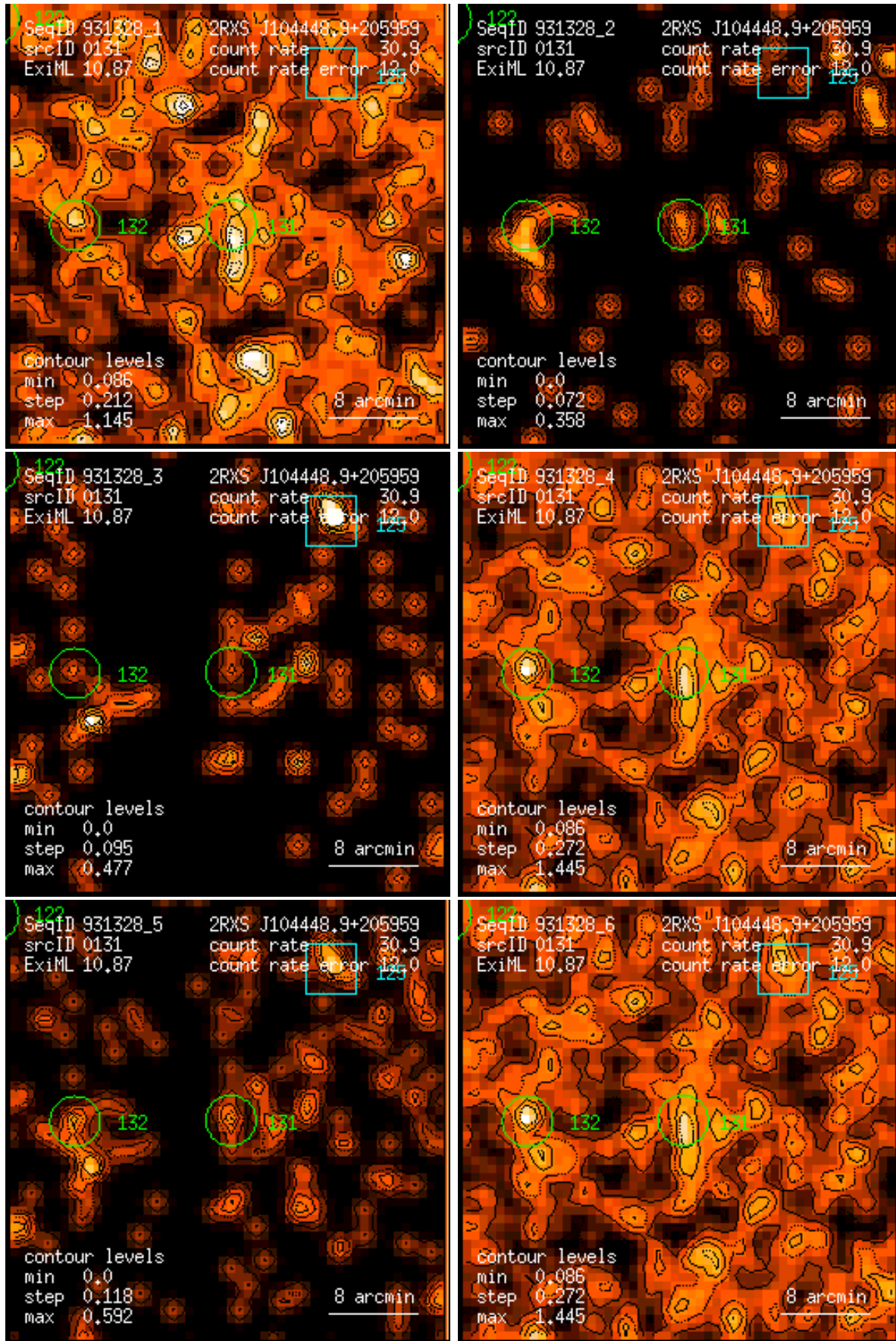
Figure 131: RASS 931328: detection 0131: band rate images, Gaussian filter: (1) PSPC channels 11 – 41, (2) 52 – 90, (3) 91 – 201, (4) 11 – 235, (5) 52 – 201, (6) 11 – 201. Broad band rates in counts/ks. Band rate contour levels in counts/ks/arcmin 2 .
