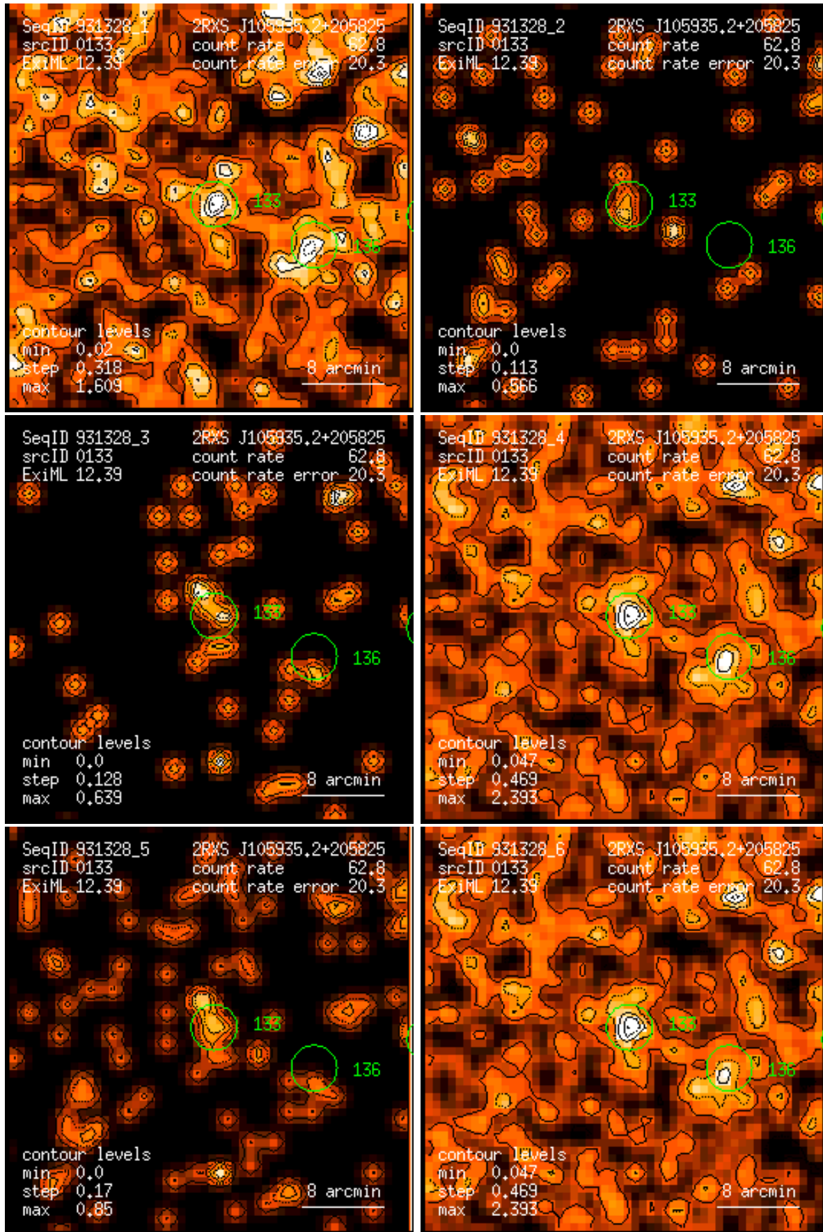
Figure 133: RASS 931328: detection 0133: band rate images, Gaussian filter: (1) PSPC channels 11 – 41, (2) 52 – 90, (3) 91 – 201, (4) 11 – 235, (5) 52 – 201, (6) 11 – 201. Broad band rates in counts/ks. Band rate contour levels in counts/ks/arcmin 2 .
