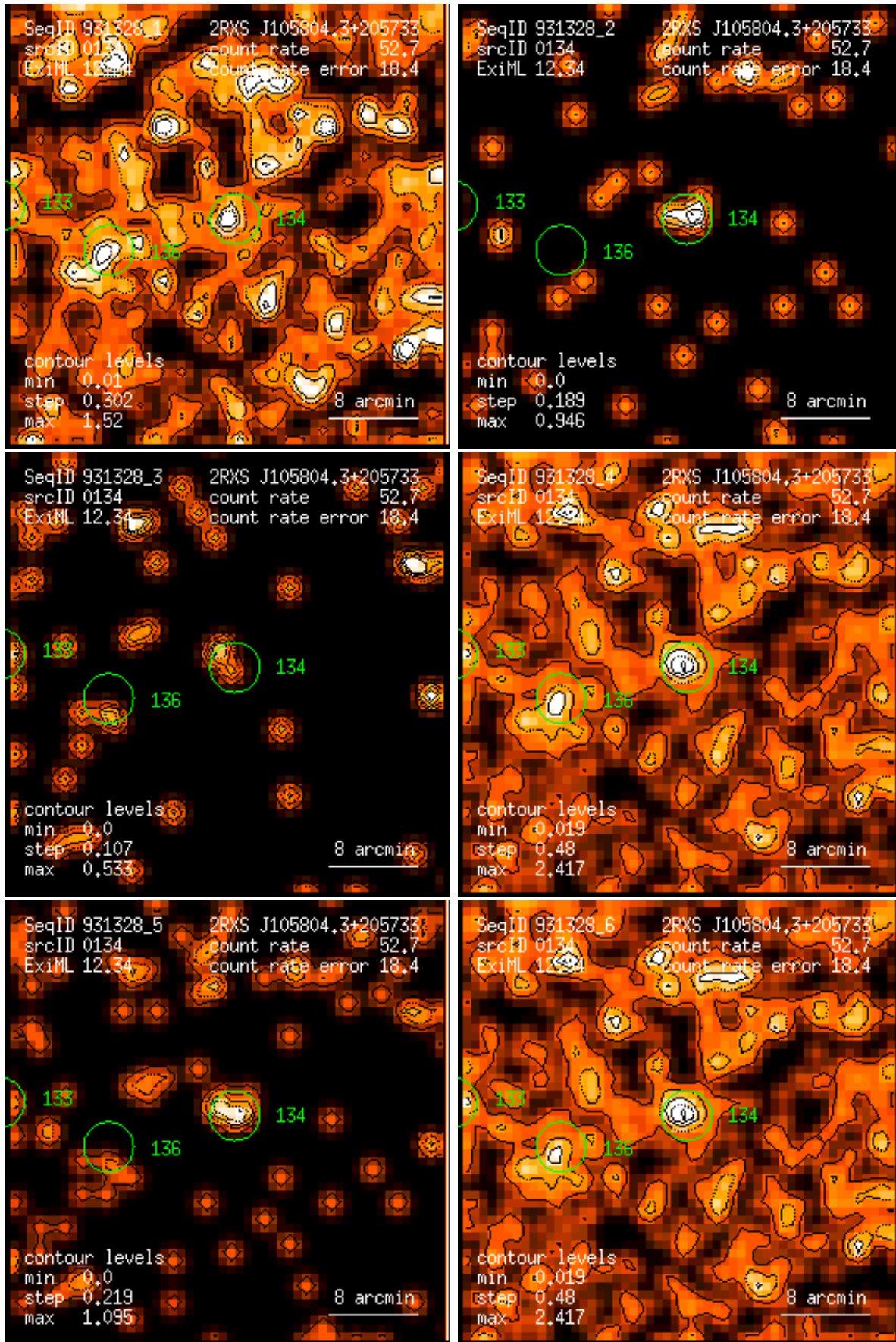
Figure 134: RASS 931328: detection 0134: band rate images, Gaussian filter: (1) PSPC channels 11 – 41, (2) 52 – 90, (3) 91 – 201, (4) 11 – 235, (5) 52 – 201, (6) 11 – 201. Broad band rates in counts/ks. Band rate contour levels in counts/ks/arcmin 2 .
