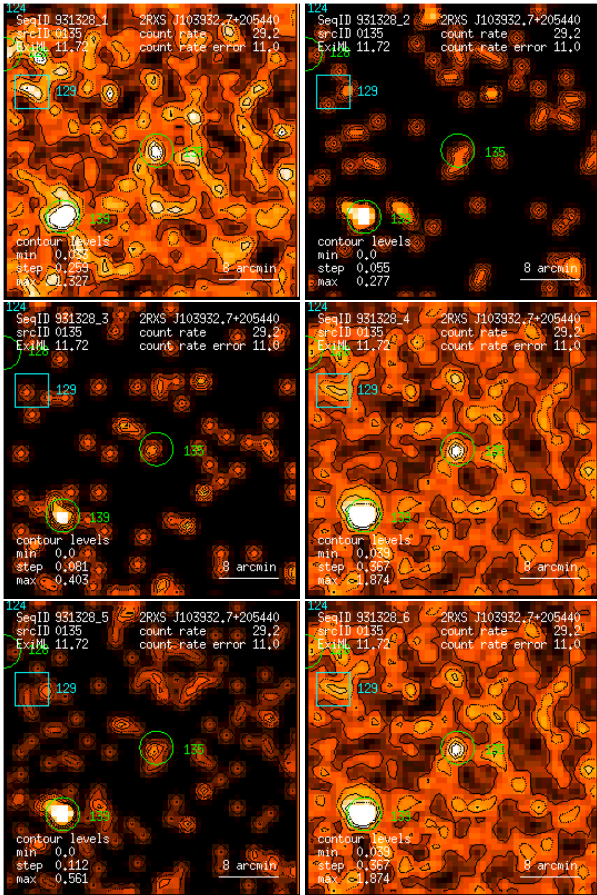
Figure 135: RASS 931328: detection 0135: band rate images, Gaussian filter: (1) PSPC channels 11 – 41, (2) 52 – 90, (3) 91 – 201, (4) 11 – 235, (5) 52 – 201, (6) 11 – 201. Broad band rates in counts/ks. Band rate contour levels in counts/ks/arcmin 2 .
