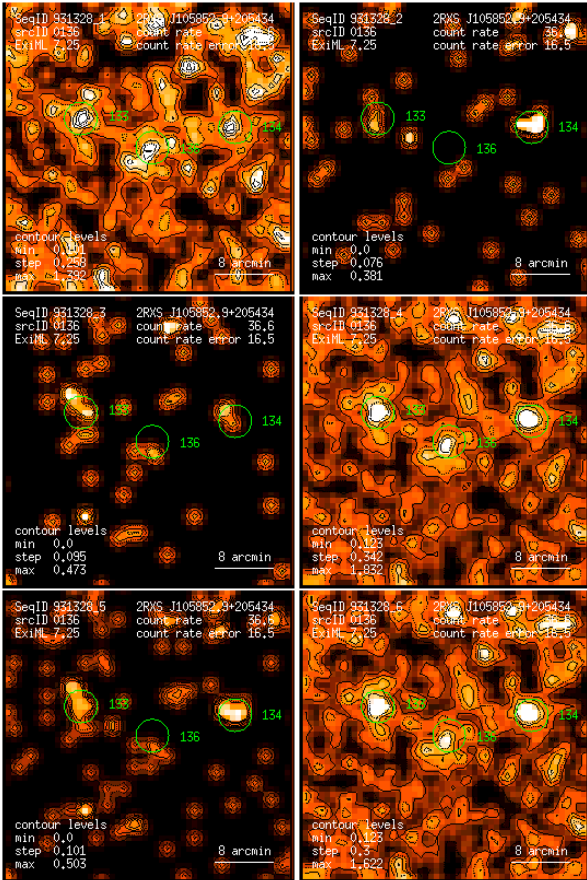
Figure 136: RASS 931328: detection 0136: band rate images, Gaussian filter: (1) PSPC channels 11 – 41, (2) 52 – 90, (3) 91 – 201, (4) 11 – 235, (5) 52 – 201, (6) 11 – 201. Broad band rates in counts/ks. Band rate contour levels in counts/ks/arcmin 2 .
