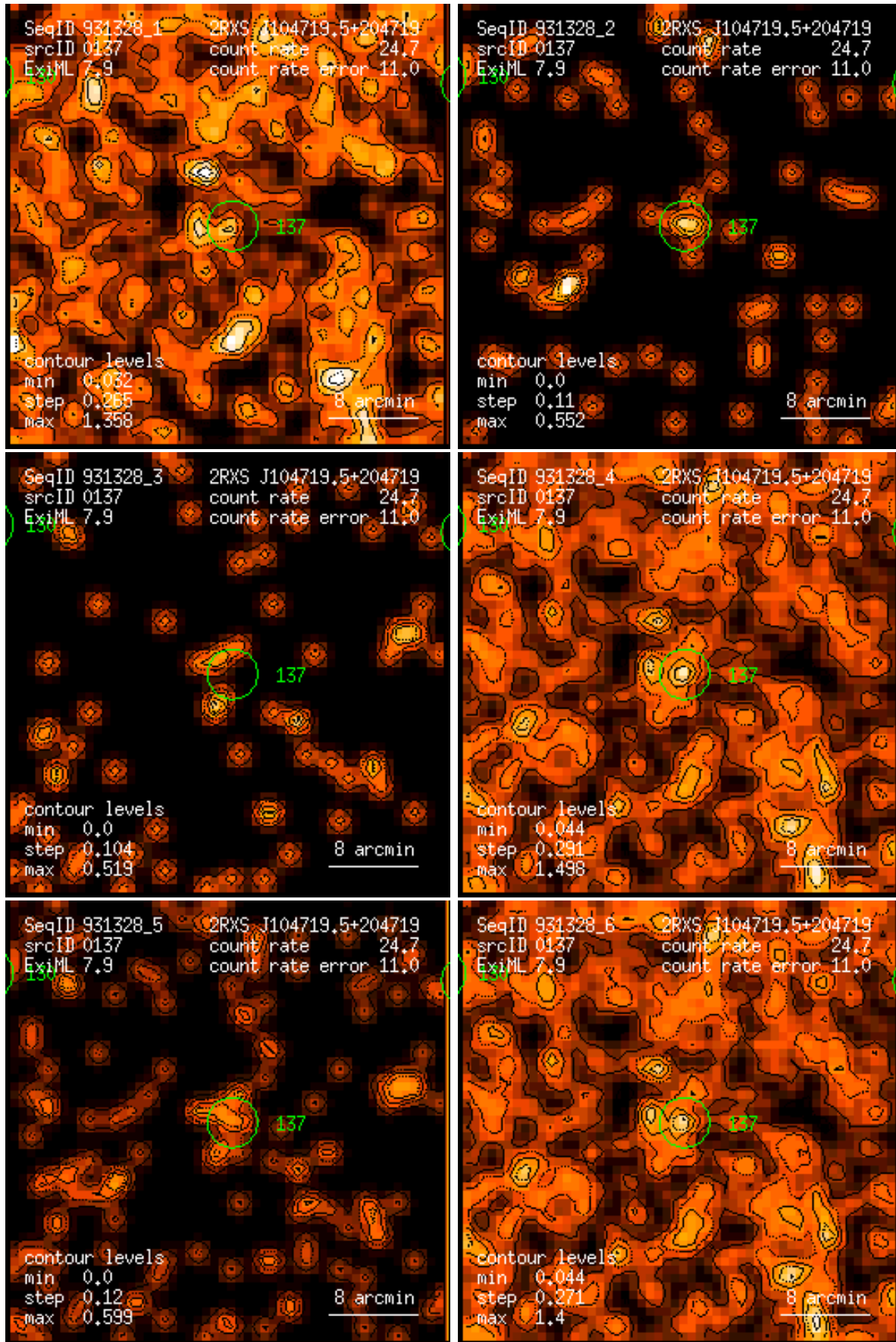
Figure 137: RASS 931328: detection 0137: band rate images, Gaussian filter: (1) PSPC channels 11 – 41, (2) 52 – 90, (3) 91 – 201, (4) 11 – 235, (5) 52 – 201, (6) 11 – 201. Broad band rates in counts/ks. Band rate contour levels in counts/ks/arcmin 2 .
