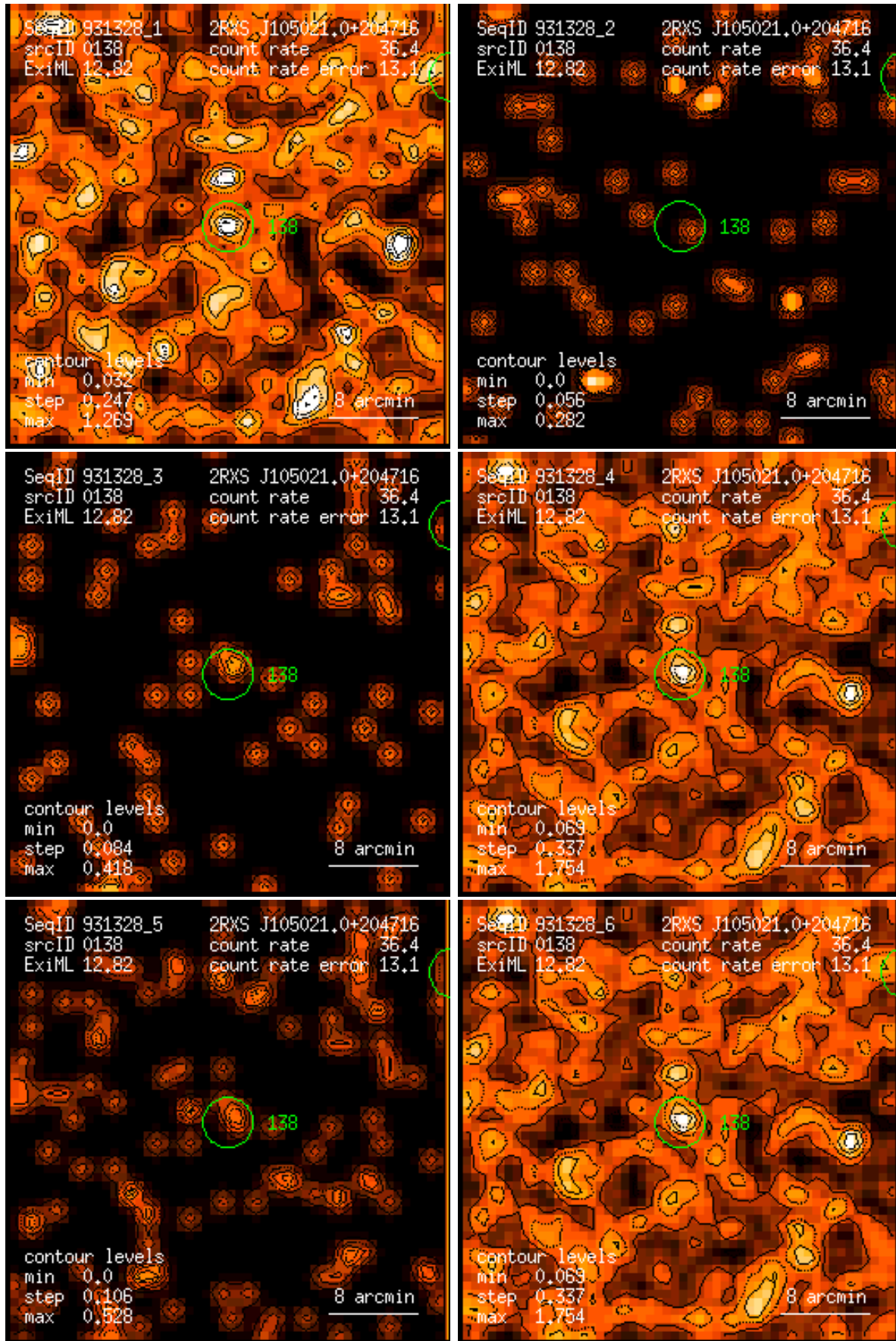
Figure 138: RASS 931328: detection 0138: band rate images, Gaussian filter: (1) PSPC channels 11 – 41, (2) 52 – 90, (3) 91 – 201, (4) 11 – 235, (5) 52 – 201, (6) 11 – 201. Broad band rates in counts/ks. Band rate contour levels in counts/ks/arcmin 2 .
