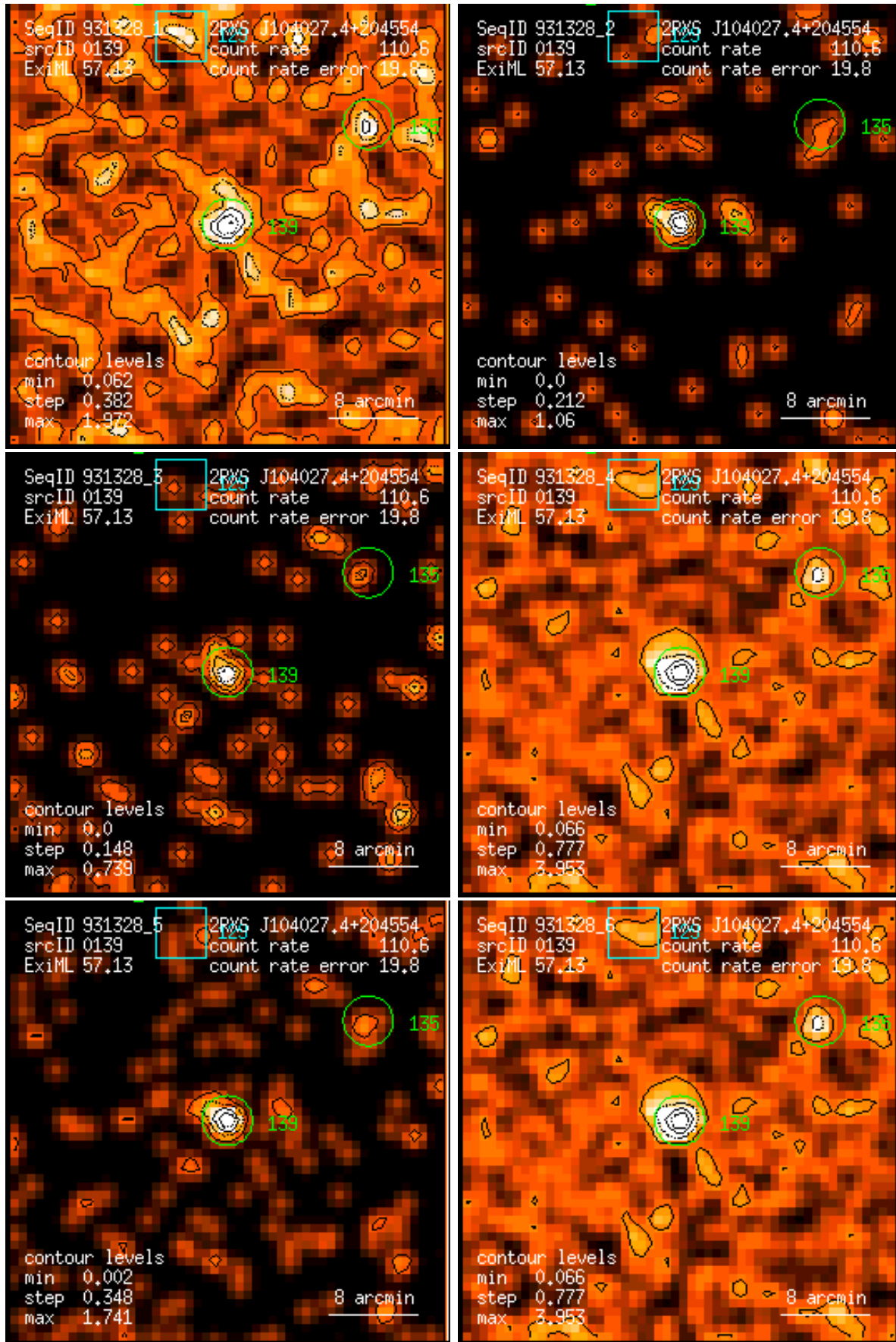
Figure 139: RASS 931328: detection 0139: band rate images, Gaussian filter: (1) PSPC channels 11 – 41, (2) 52 – 90, (3) 91 – 201, (4) 11 – 235, (5) 52 – 201, (6) 11 – 201. Broad band rates in counts/ks. Band rate contour levels in counts/ks/arcmin 2 .
